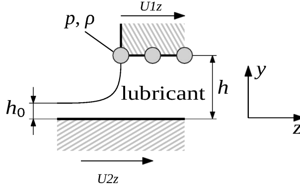
Figure 16.4: assumptions for partially flooded boundaries of the bearing
