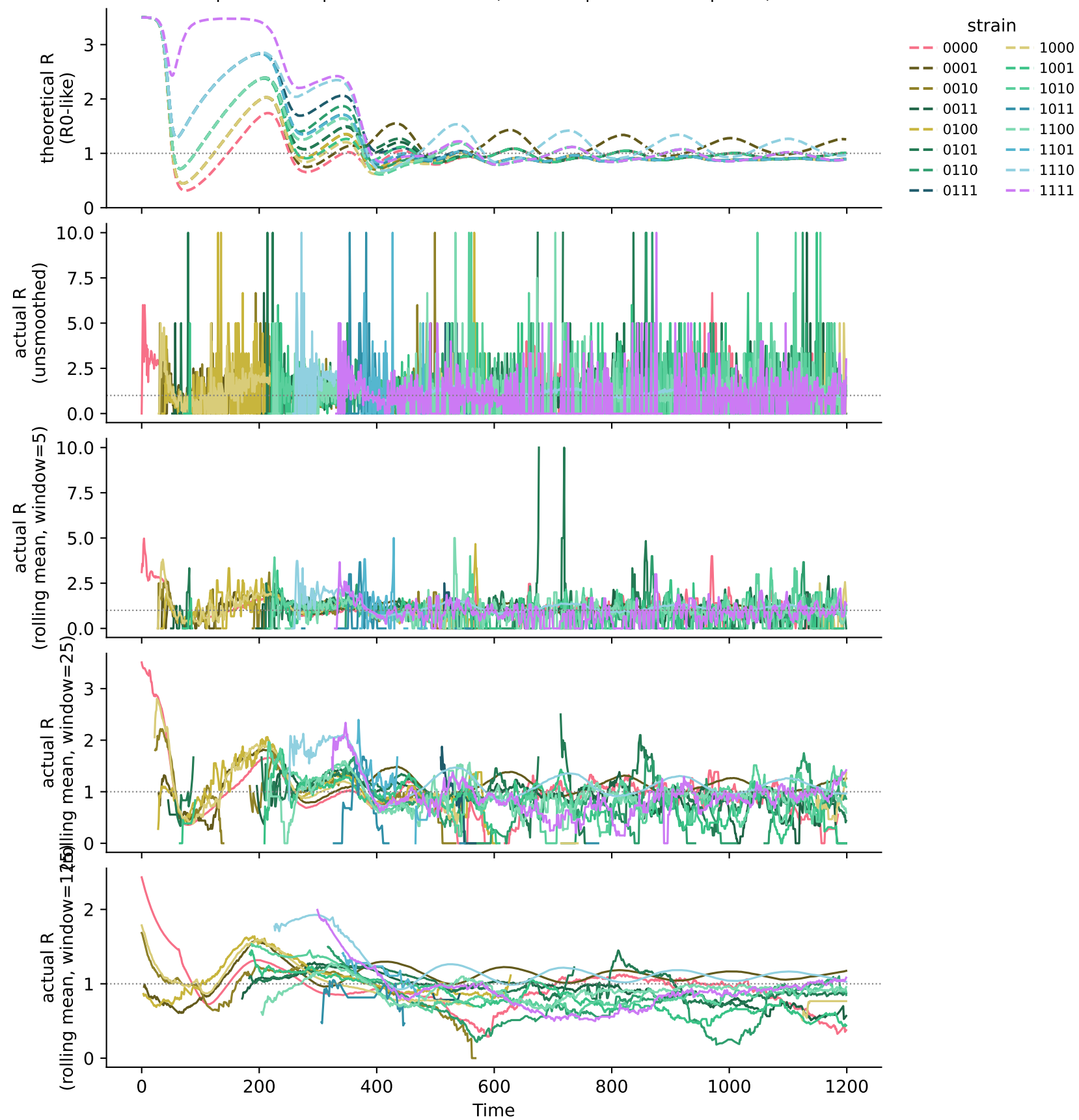
per-strain reproduction number (scaled to per-infectious-period)
