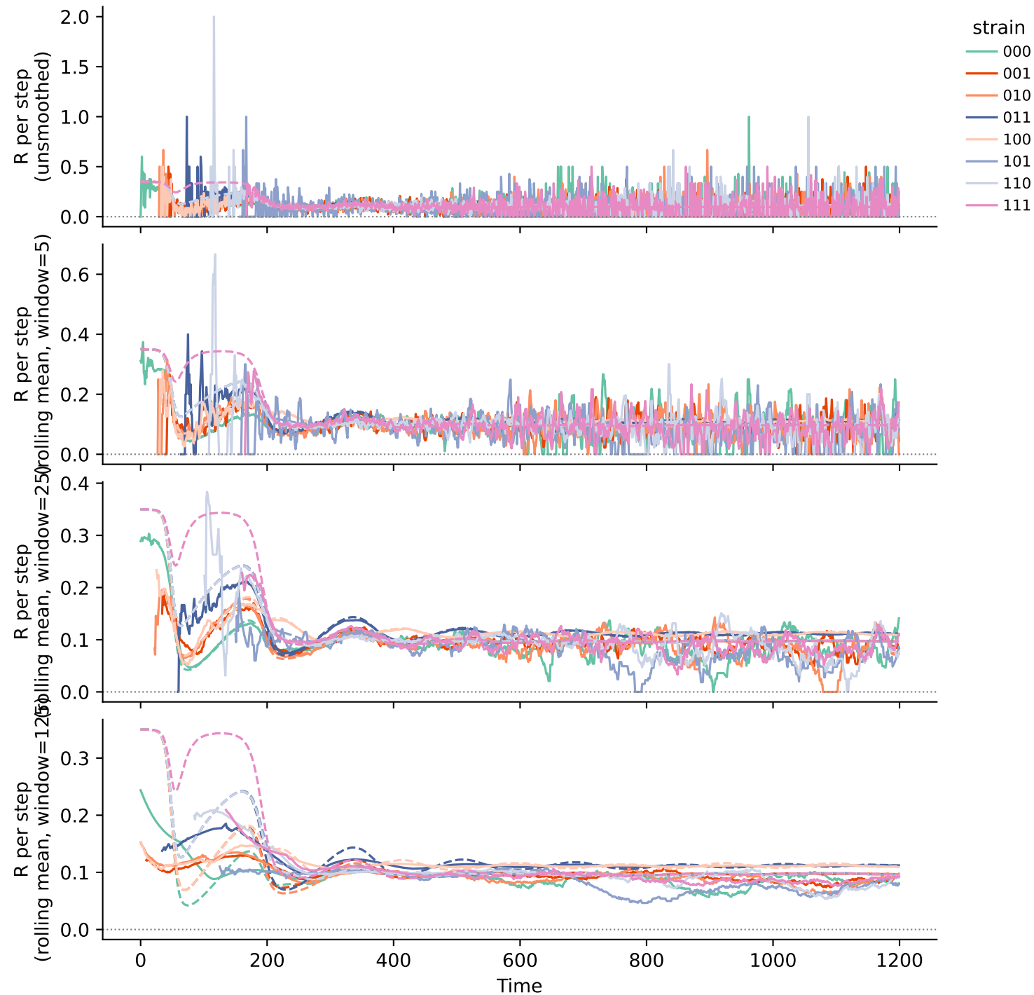
actual (solid) vs. theoretical (dashed) per-strain new infections per current infected per step
