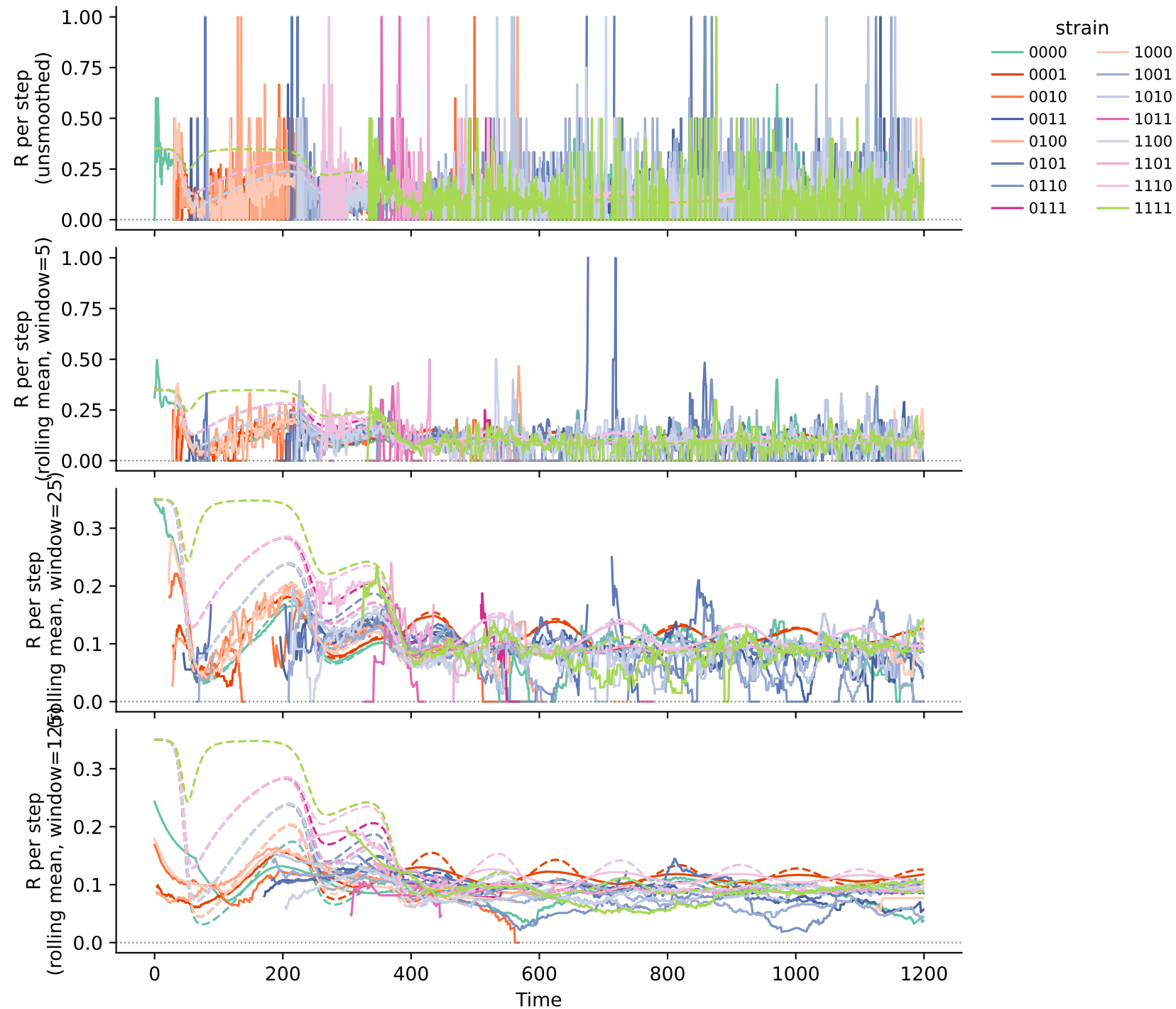
actual (solid) vs. theoretical (dashed) per-strain new infections per current infected per step
