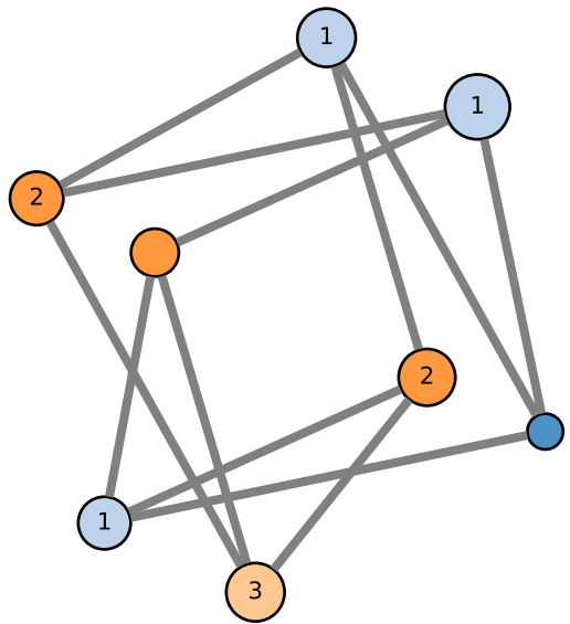
n = 1
