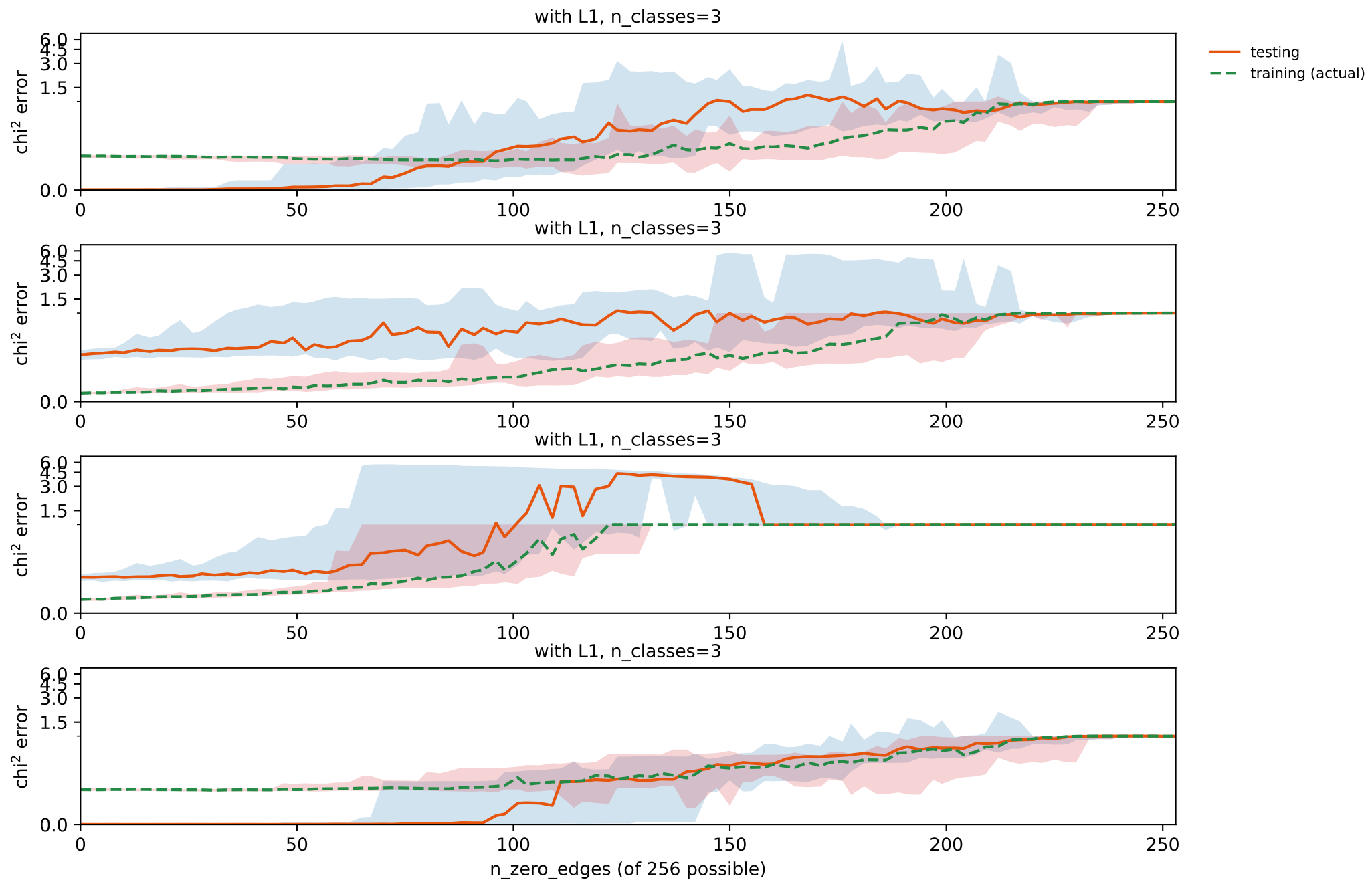
final testing / training (actual) \chi^2 error vs. n_zero_edges
