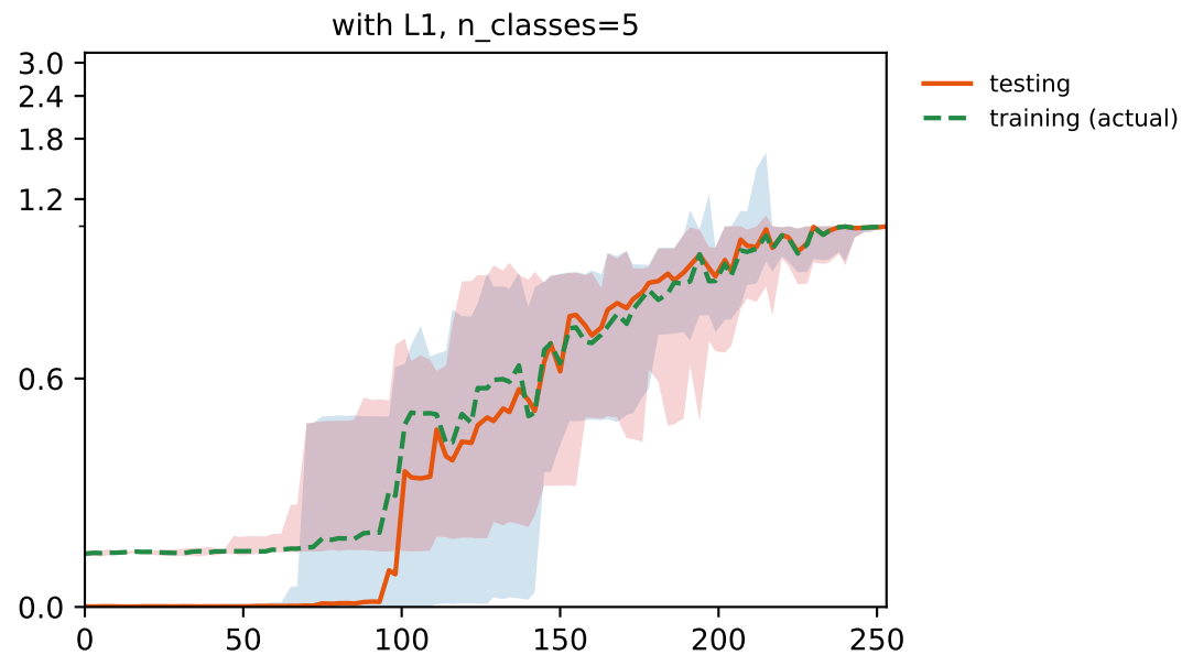
final testing / training (actual) \chi^2 error vs. n\_zero\_edges
