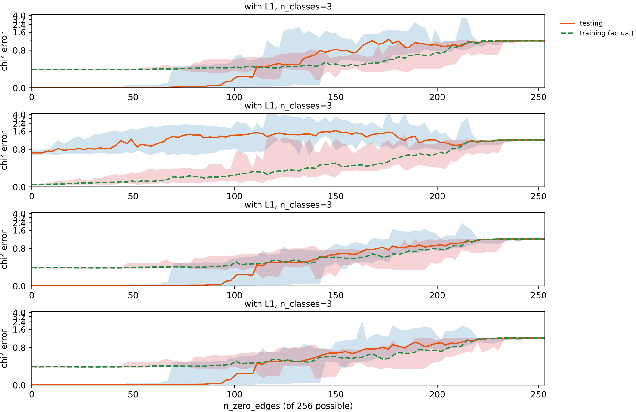
final testing / training (actual) \chi^2 error vs. n_{\text{zero\_edges}}
