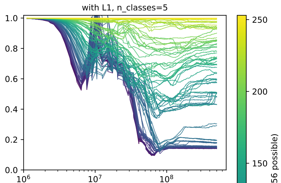
training (actual) \chi^2 error over evolutionary time
