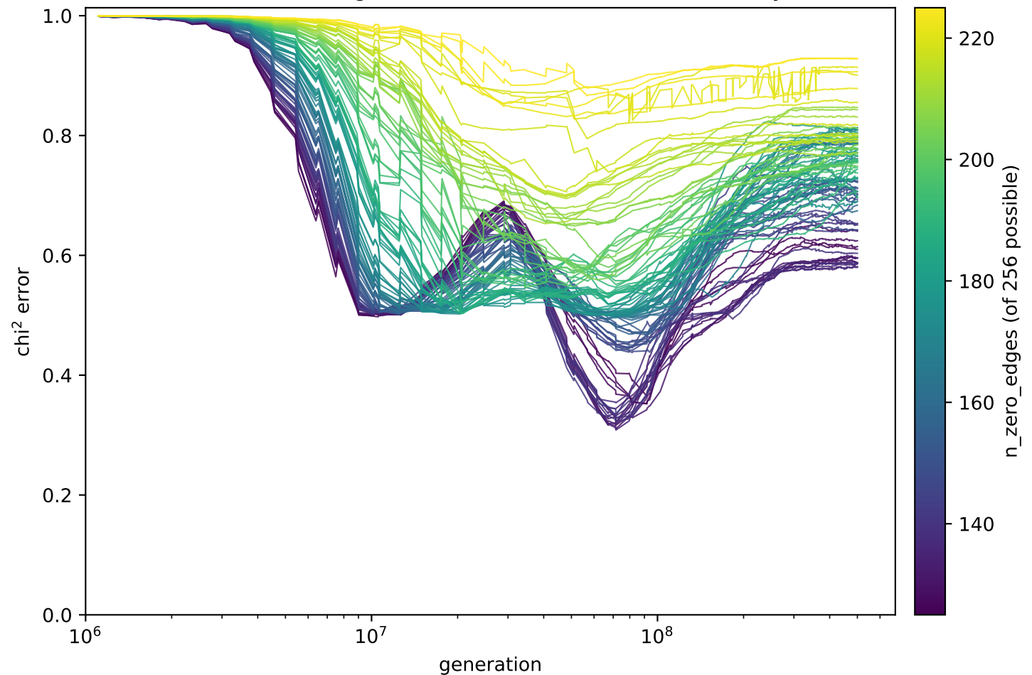
doubled-S1: training (actual) \chi^2 error over evolutionary time
