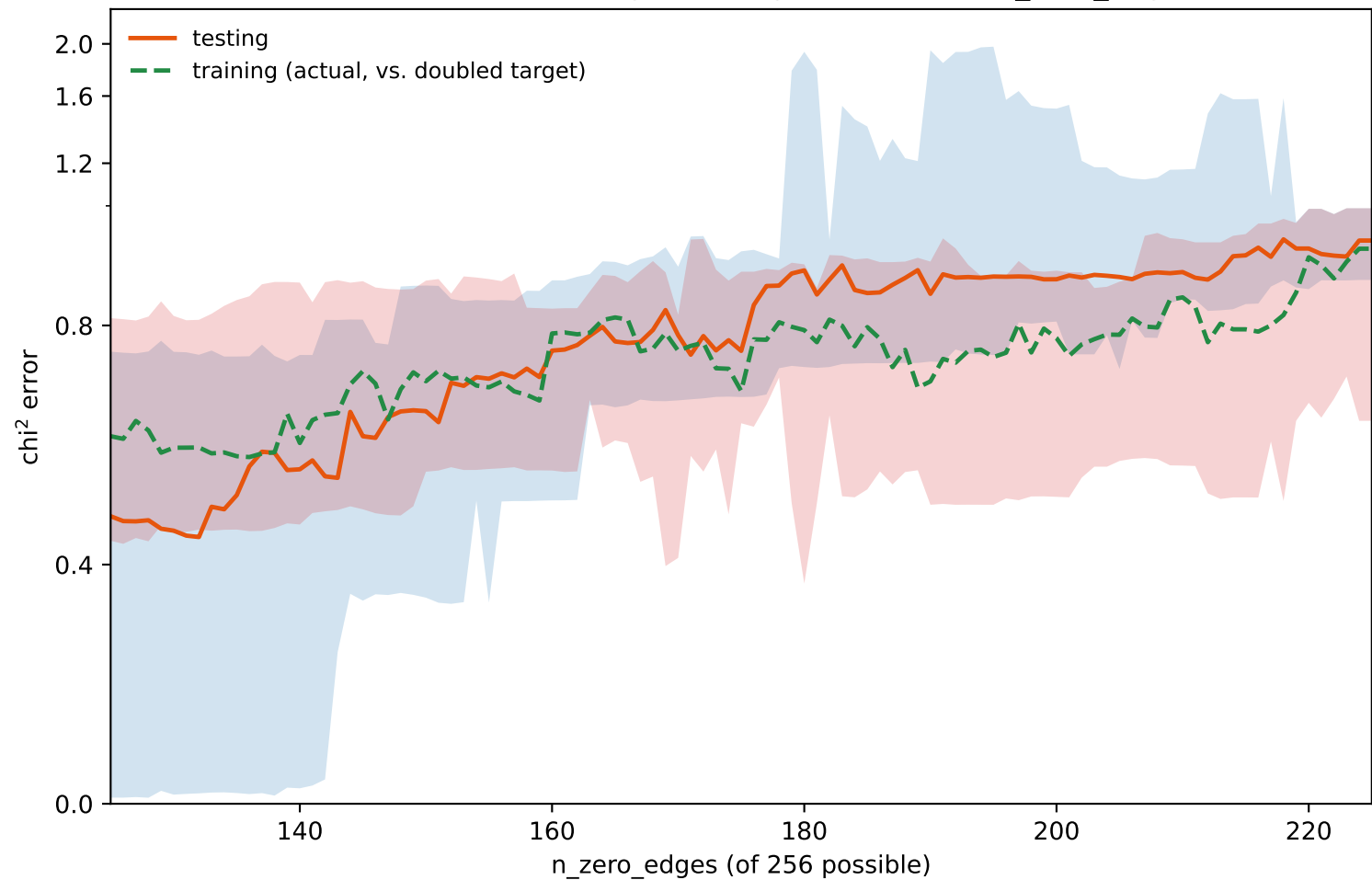
doubled-S1: final testing / training chi 2 error vs. n_zero_edges
