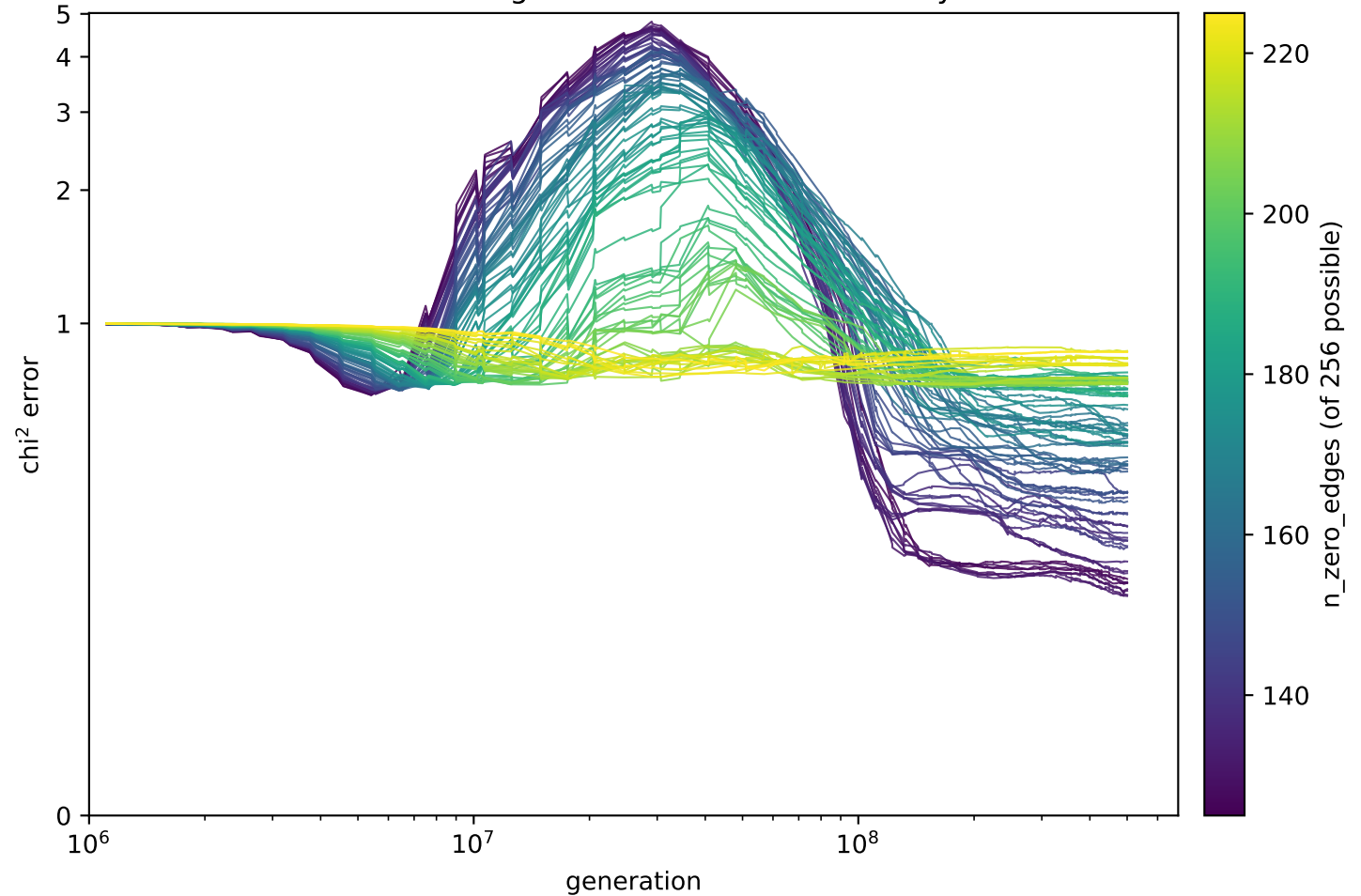
doubled-S1: testing \chi^2 error over evolutionary time
