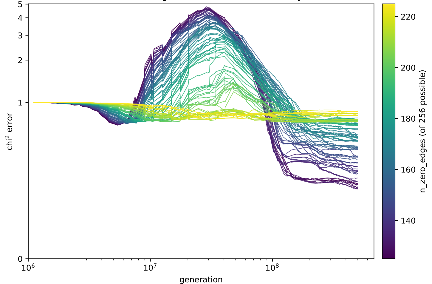
doubled-S1: testing \chi^2 error over evolutionary time
