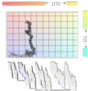
sample lineage
