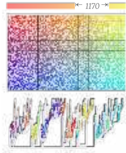
reconstructed phylogeny
