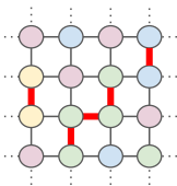
graph coloring
