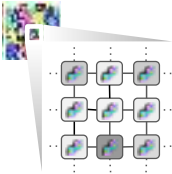
digital evolution
