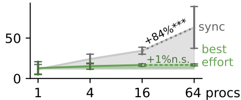
Graph Color (solution error)
