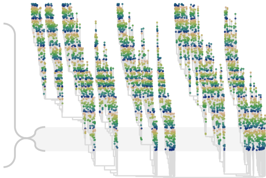
Reconstructed Phylogeny
