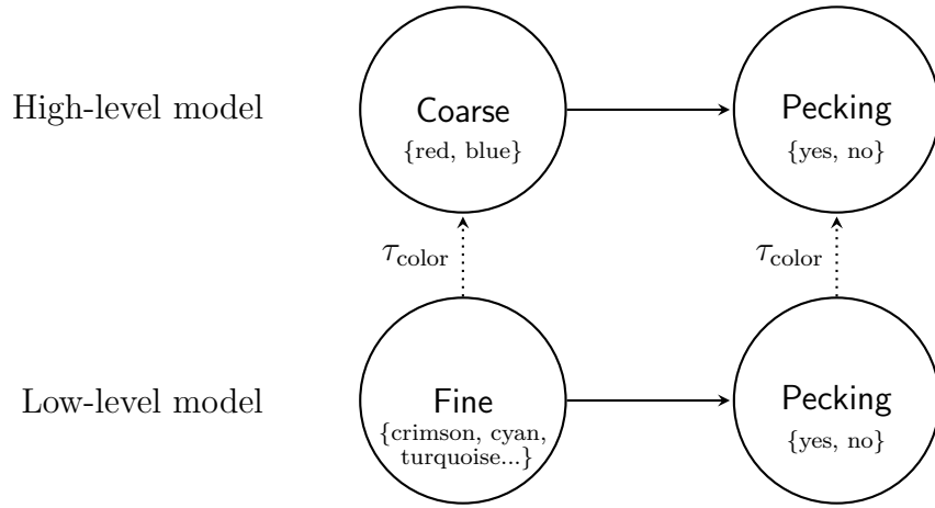
Figure 1: Color as an abstraction. An alignment \tau_{\text{color}} maps values of the Fine color variable (crimson, scarlet) to values of the Coarse color variable (red). Solid arrows express causal relationships, e.g. that intervening on the value of the Coarse color variable can change the value of Pecking .
