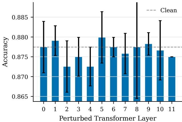
Accuracy by Noise Injection Layer (std. dev. = 0.2)
