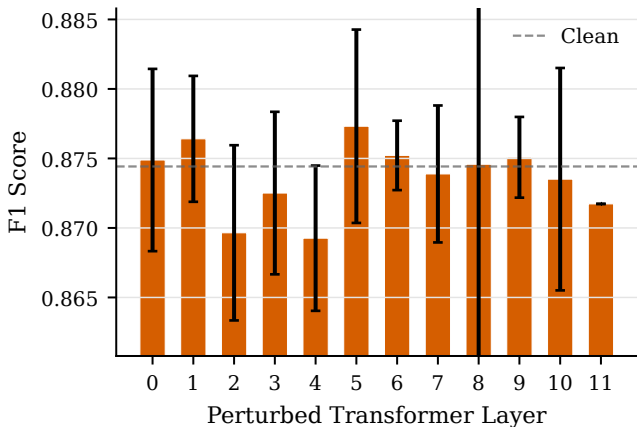
F1 Score by Noise Injection Layer (std. dev. = 0.2)
