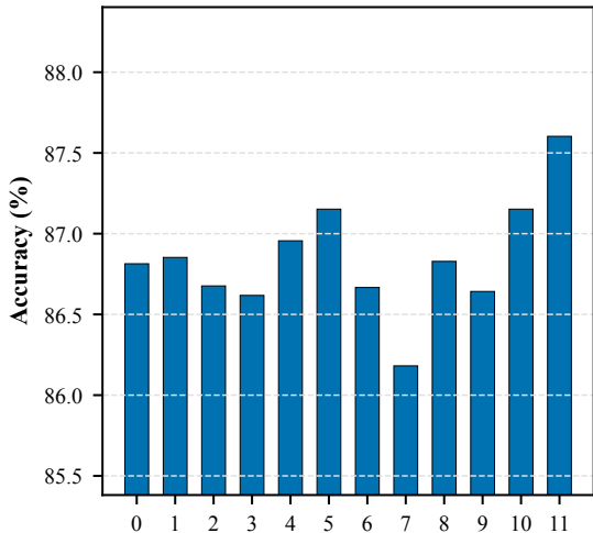
Accuracy by Noise Injection Layer (std. dev. = 0.4)
