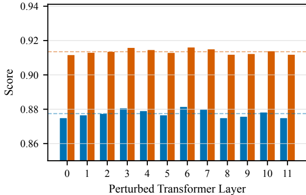
(b) Single-layer noise position
