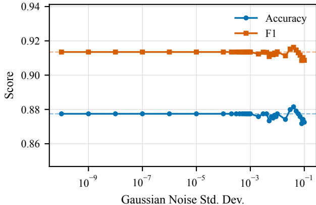
(a) Uniform layer-output noise
