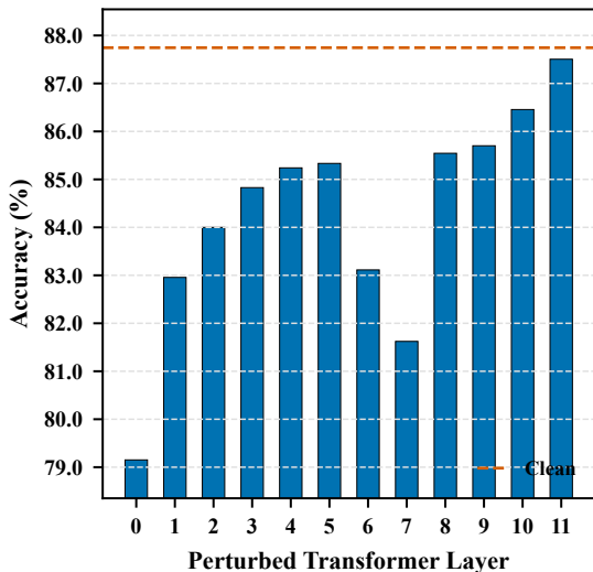
Accuracy by Noise Injection Layer (std. dev. = 0.6)
