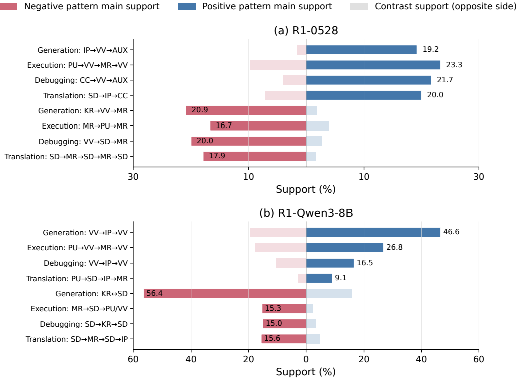
Fig. 2. Support Comparison between Positive and Negative Patterns.
