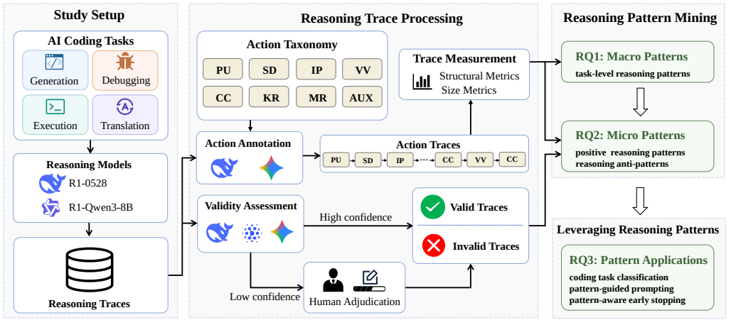
Fig. 1. Overview of the reasoning-pattern analysis framework.
