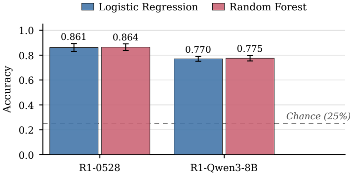
Fig. 3. Task identification from reasoning pattern features.
