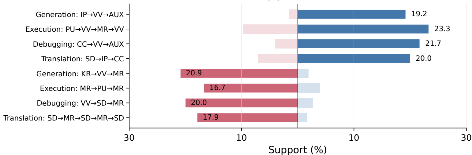
(a) R1-0528
