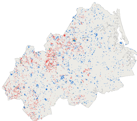
GLM suitability (lulcc) / Ordered FoM 0.029
