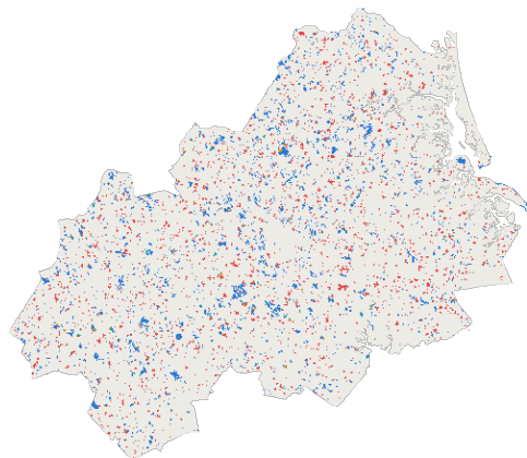
logistic regression / CLUMPY FoM 0.026
