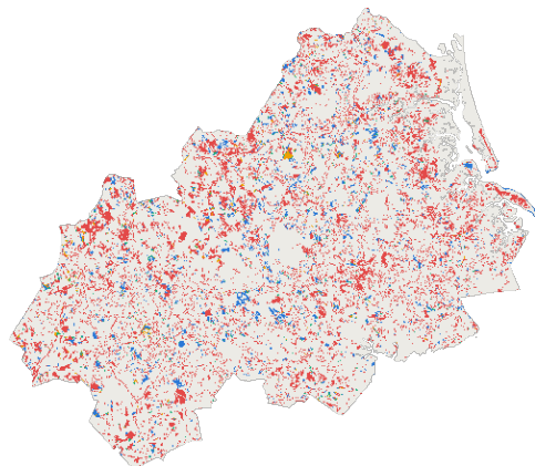
GLM suitability (lulcc) / CLUE-S FoM 0.033
