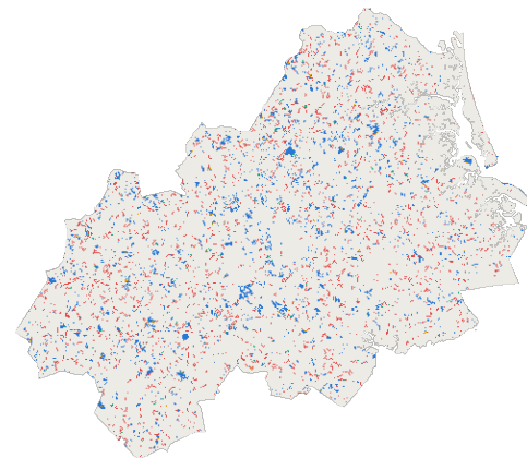
Weights of Evidence / Dinamica FoM 0.029
