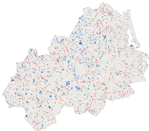
random forest / Dinamica FoM 0.035
