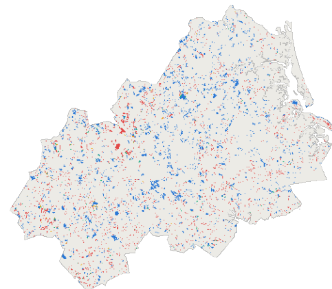
logistic suitability (CLUinPy) / CLUMondo FoM 0.033
