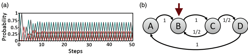
Figure 8.8 The state diagram of case H. (a) The behavior of the system on 50 steps. The orange line represents the probability that the system will be in state “A”. The blue line represents the probability that the system will be in state “B”. The gray line represents the probability that the system will be in state “C”. The burgundy line represents the probability that the system will be in state “D”. (b) The state diagram of case H. The red arrow indicates the state (the jar) from which the first draw begins.
