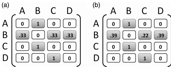
Figure 9.7 The verification of the output. (a) Initial transition matrix ( T1 ) of the simulator. (b) Transition probabilities between letters of the output presented in the form of a transition matrix ( T2 ).
