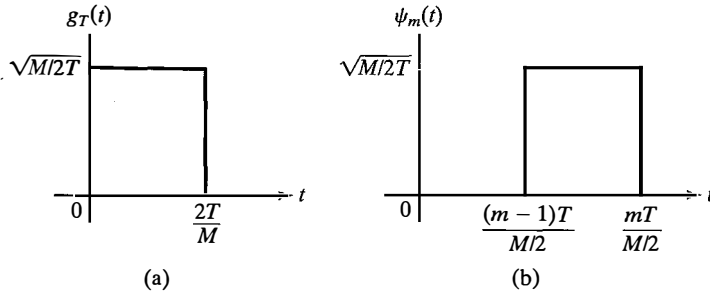
Figure 9.4 Rectangular pulse g_T(t) and basis function \psi_m(t) for M -ary biorthogonal PPM signal waveforms.
