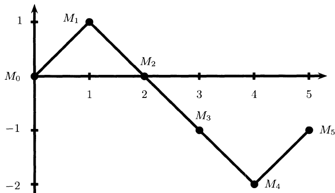
Fig. 5.1.1. Five steps of a random walk
