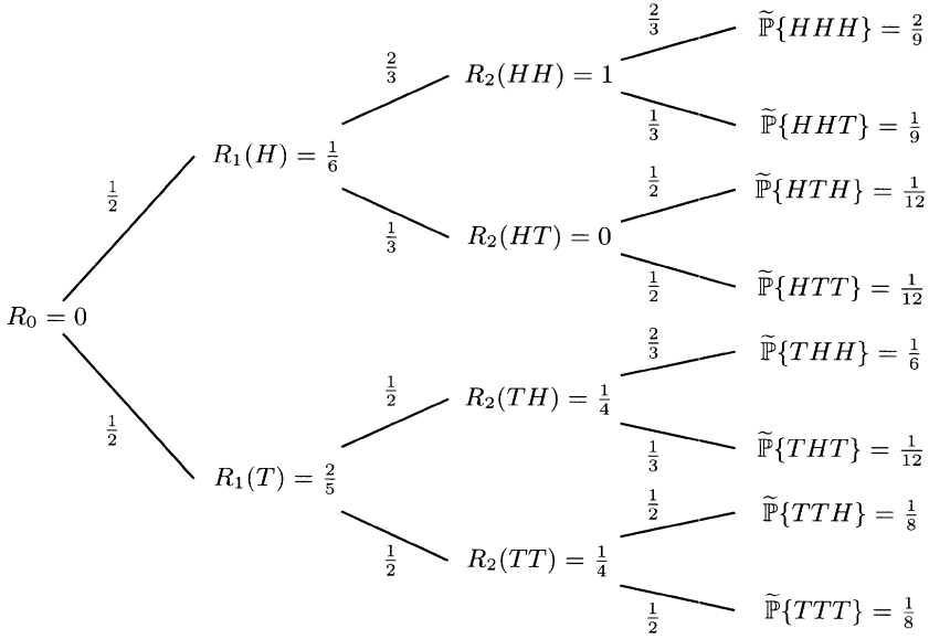
Fig. 6.3.1. A three-period interest rate model.
