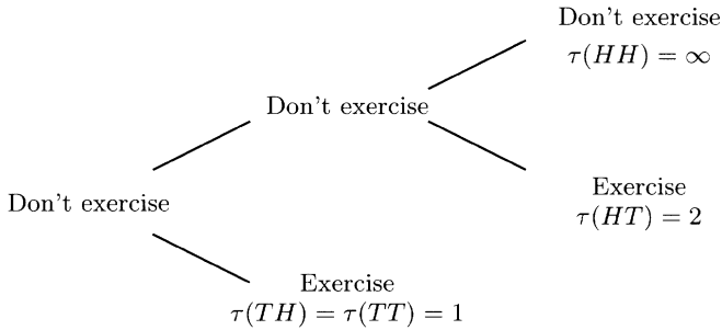
Fig. 4.3.1. Exercise rule \tau .
