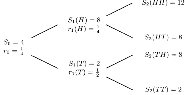
Fig. 2.8.1. A stochastic volatility, random interest rate model.
