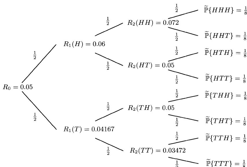
Fig. 6.5.1. A three-period Black-Derman-Toy interest rate model.
