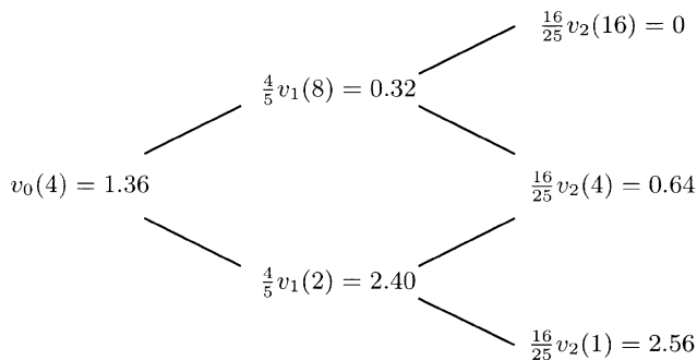
Fig. 4.2.3. Discounted American put prices.
