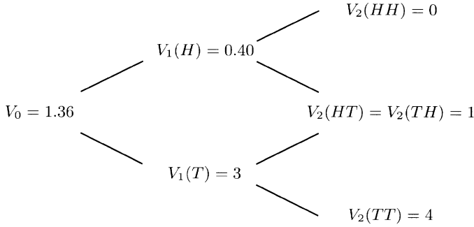
Fig. 4.4.2. American put prices.
