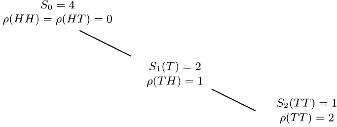
Fig. 4.3.2. Exercise rule \rho .
