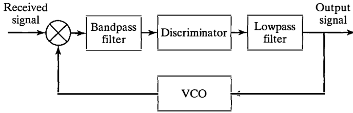
Figure 4.13 Block diagram of an FMFB demodulator.
