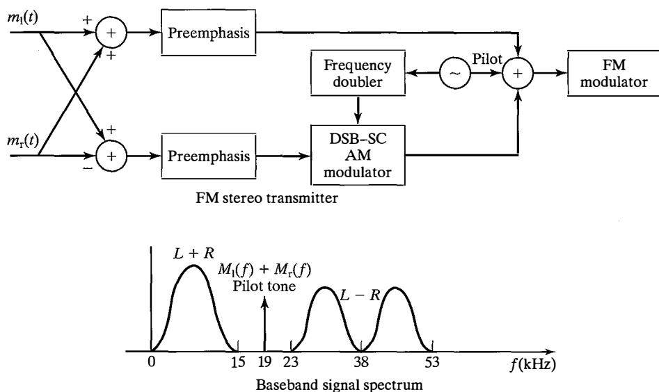
Figure 4.17 FM stereo transmitter and signal spacing.
