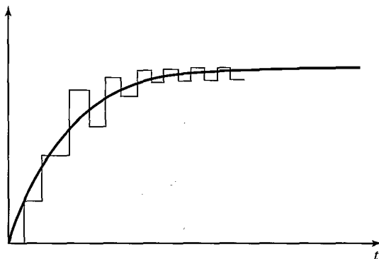
Figure 7.16 Performance of adaptive delta modulation.
