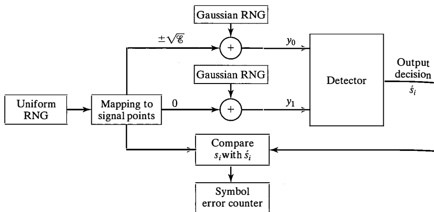
Figure CP-9.4 Simulation model for the detection of M = 4 biorthogonal signals.
