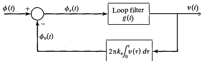
Figure 4.15 Linearized PLL.
