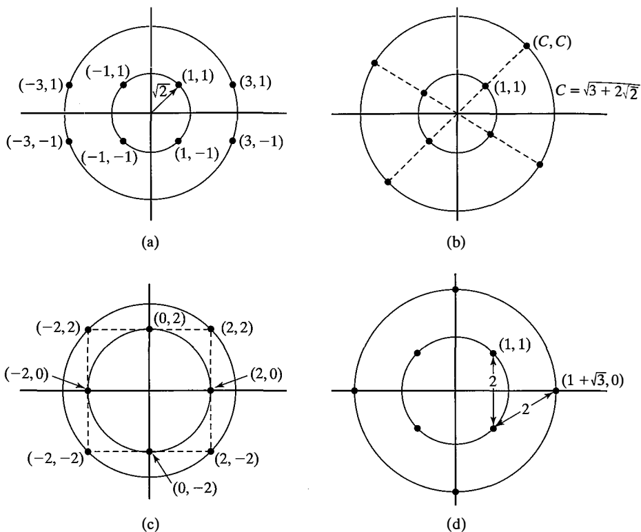
Figure 8.59 Four 8-point QAM signal constellations.
