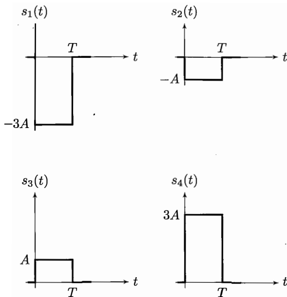
Figure 8.42 M = 4 PAM signal waveforms.
