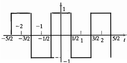
Figure 2.27 Signal x(t) in Equation (2.2.9).
