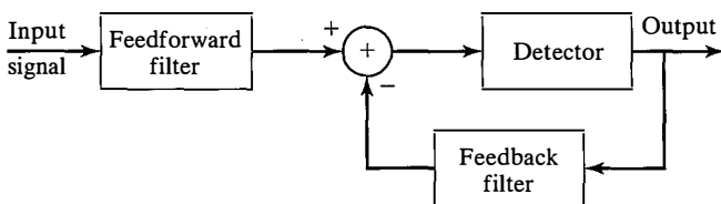
Figure 10.31 Block diagram of DFE.
