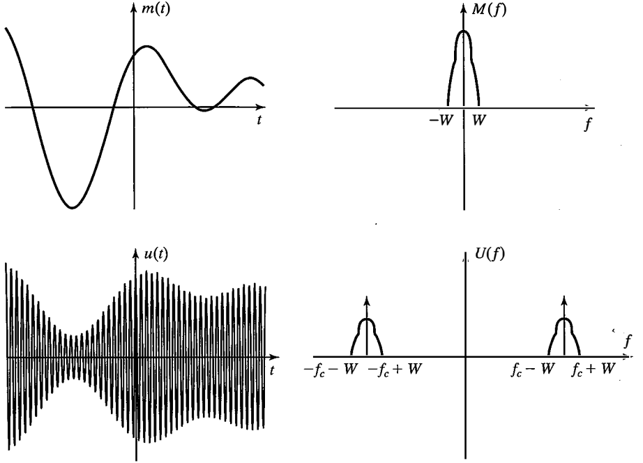
Figure 3.11 Conventional AM in both the time and frequency domain.
