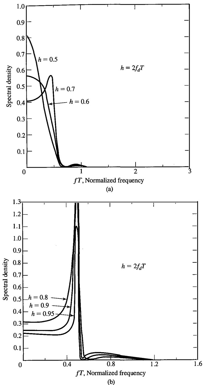
Figure 9.26 Power density spectrum of binary CPFSK.
