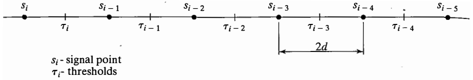
Figure 8.45 Placement of thresholds at midpoints of successive amplitude levels.
