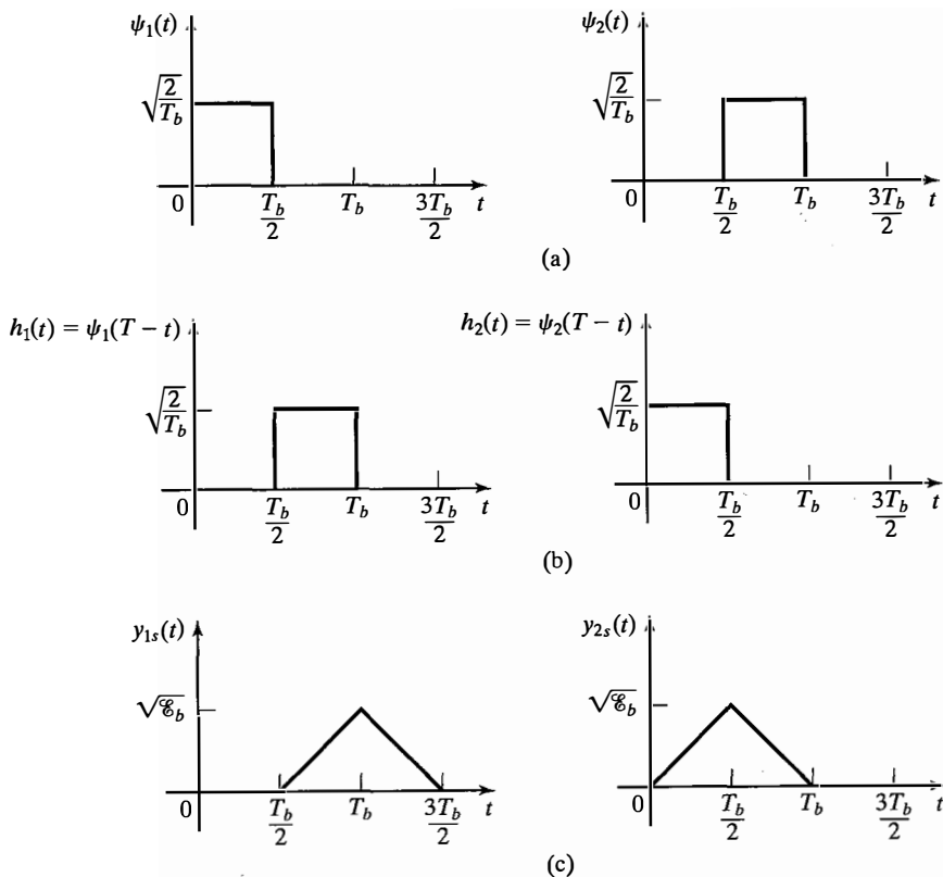
Figure 8.31 Basis functions and matched filter responses for Example 8.3.8.
