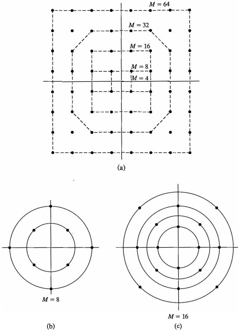
Figure 8.56 (a) Rectangular signal-space constellations for QAM. (b, c) Examples of combined PAM-PSK signal-space constellations.
