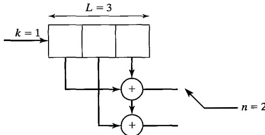
Figure 13.10 A rate \frac{1}{2} convolutional encoder.
