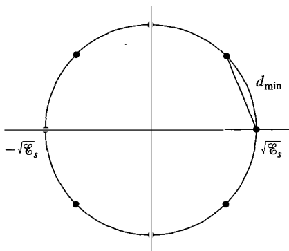
Figure 13.32 The 8-PSK constellation used for bandwidth-efficient coding.
