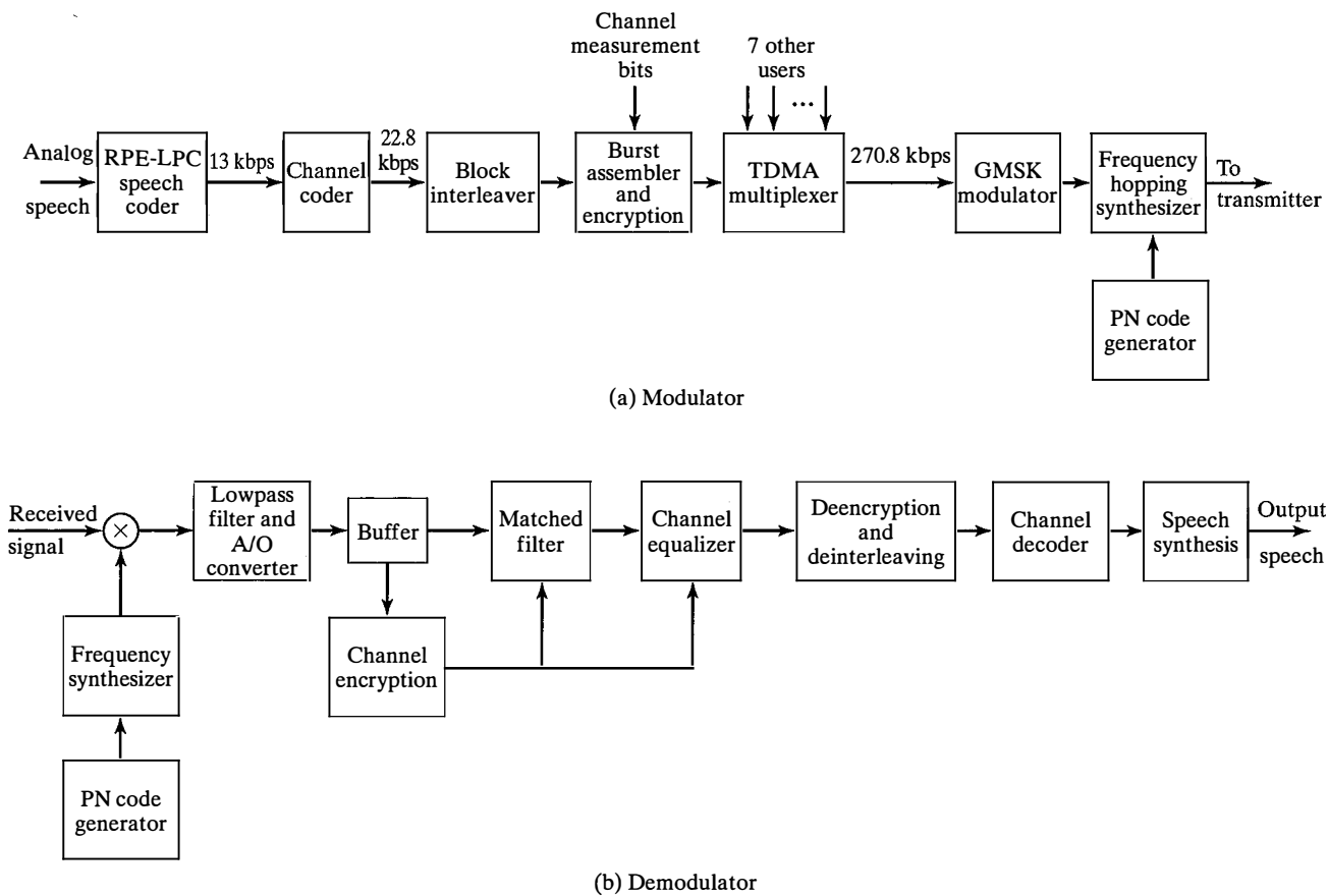
Figure 15.24 Functional block diagram of a modulator and demodulator for GSM.
