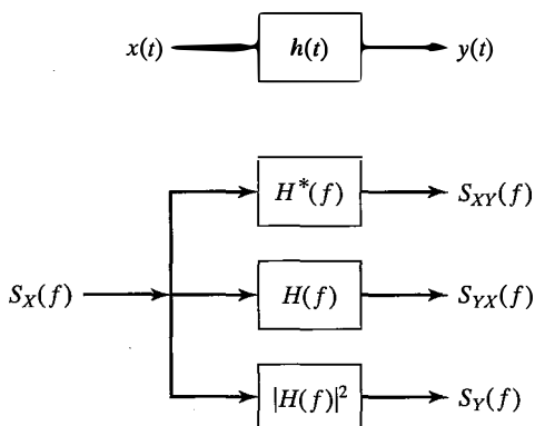
Figure 5.18 Input-output relations for the power spectral density and the cross-spectral density.
