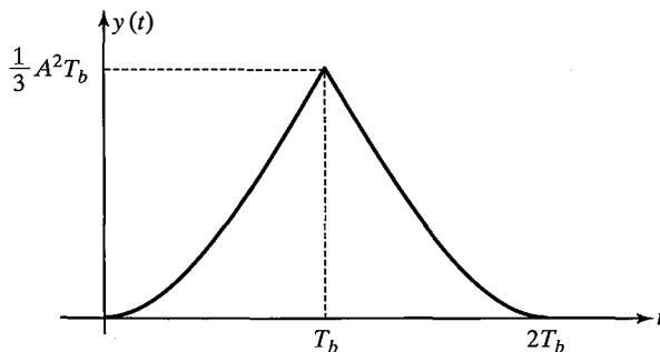
Figure 8.29 The matched filter output is the autocorrelation function s(t) .
