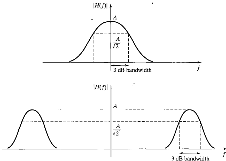
Figure 2.46 3 dB bandwidth of filters in Example 2.3.24.
