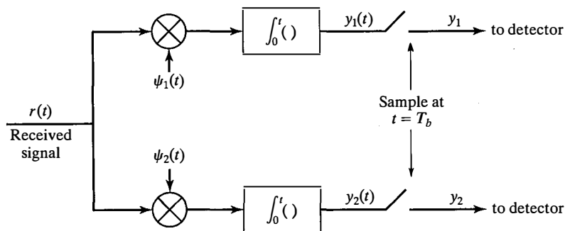
Figure 8.24 Correlation-type demodulator for binary orthogonal signals.
