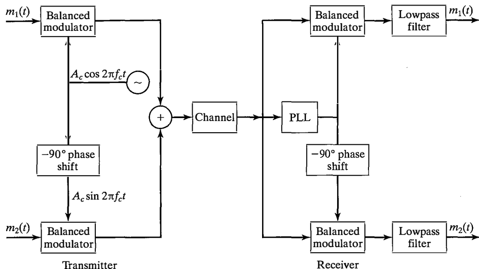
Figure 3.32 Quadrature-carrier multiplexing.
