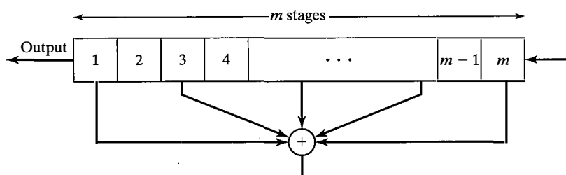
Figure 15.6 General m -stage shift register with linear feedback.
