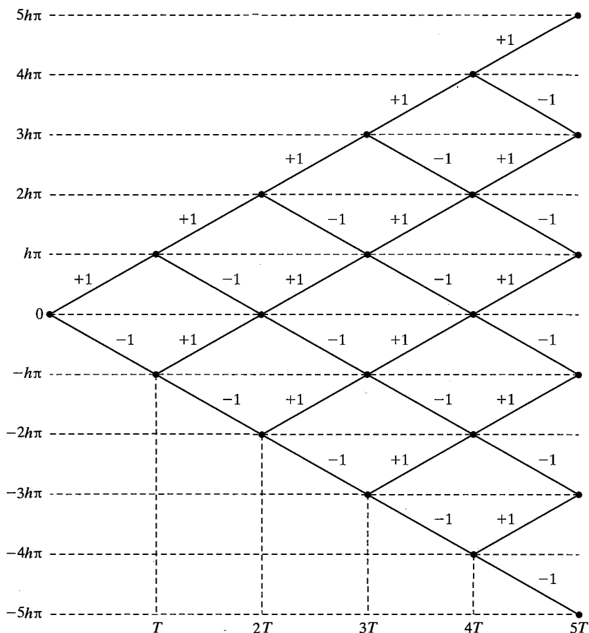
Figure 9.17 Phase trajectory for binary CPFSK.
