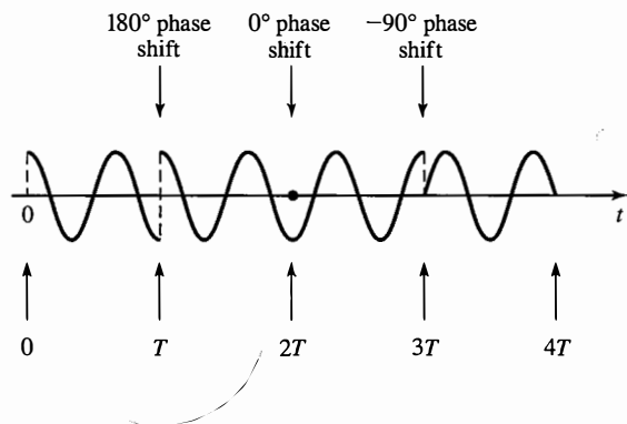
Figure 8.47 Example of a four-phase PSK signal.
