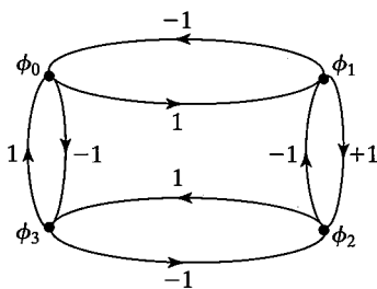
Figure 9.20 State diagram for binary CPFSK with h = 1/2 .
