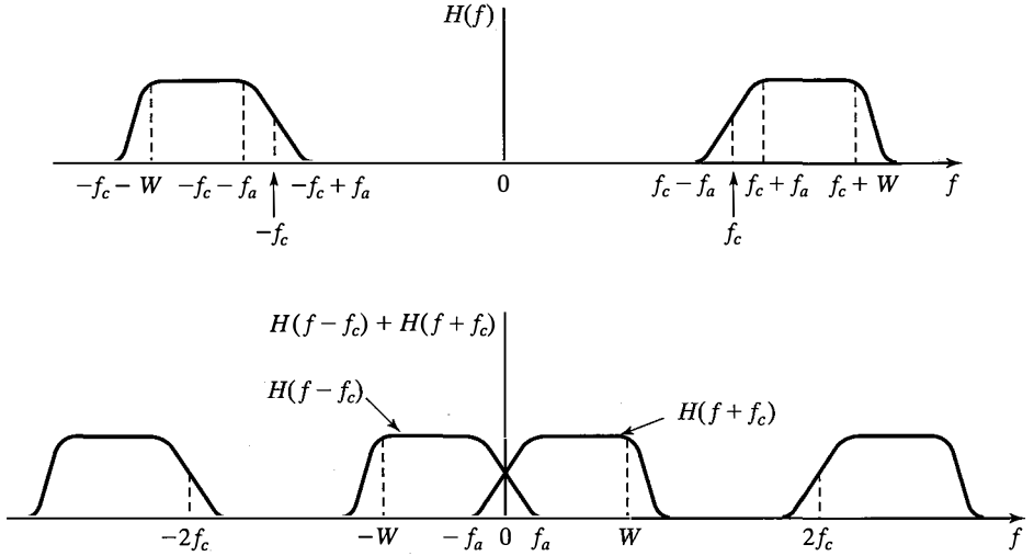
Figure 3.19 VSB filter characteristics.
