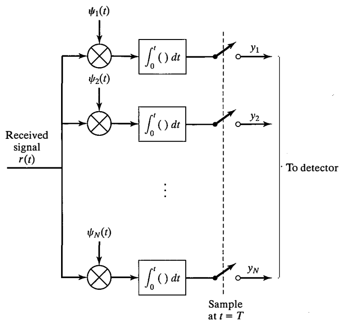
Figure 8.35 Correlation-type demodulator.
