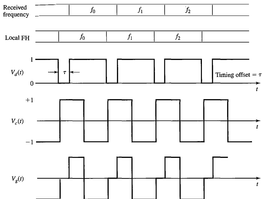
Figure 15.19 Waveforms for the tracking method of FH signals shown in Figure 15.18.
