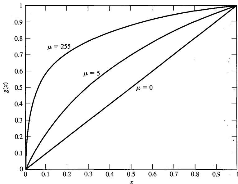
Figure 7.9 A graph of \mu -law compander characteristics.
