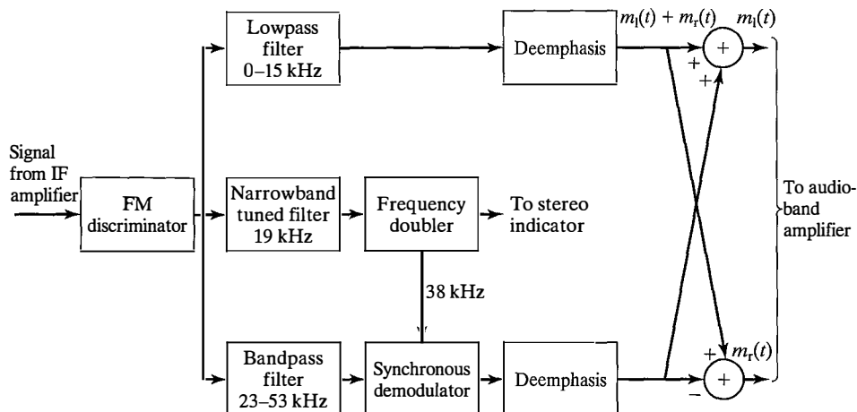
Figure 4.18 FM-stereo receiver.
