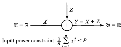
Figure 12.9 Additive white Gaussian noise channel with power constraint.
