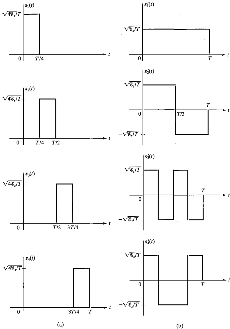
Figure 9.1 Two sets of M = 4 orthogonal signal waveforms.
