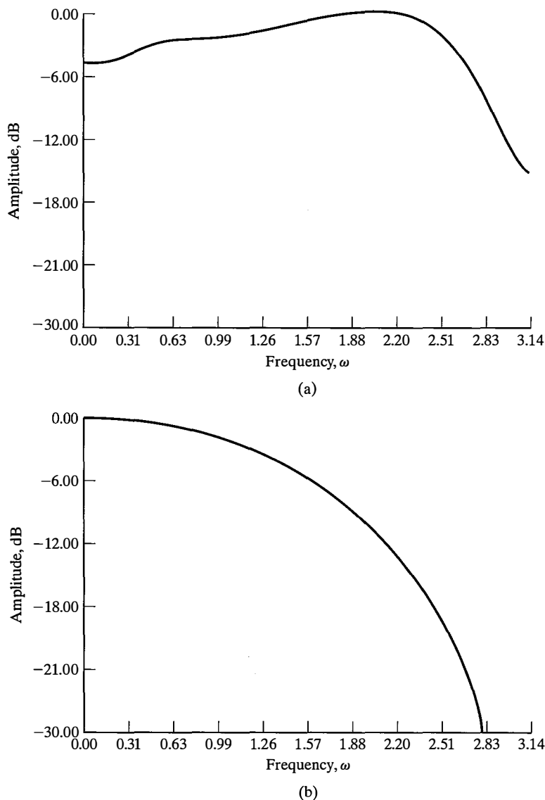
Figure 10.29 Amplitude spectra for (a) channel A shown in Figure 10.28(a) and (b) channel B shown in Figure 10.28(b).
