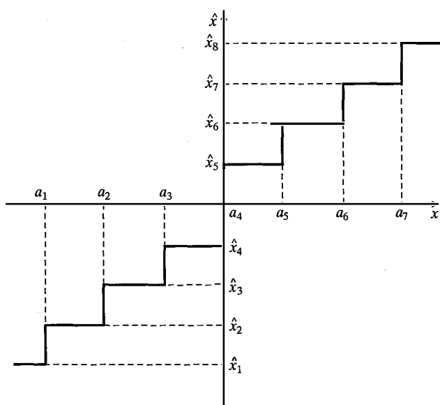
Figure 7.3 Example of an eight-level quantization scheme
