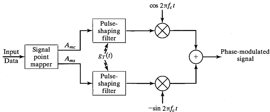
Figure 8.48 Block diagram of a digital-phase modulator.
