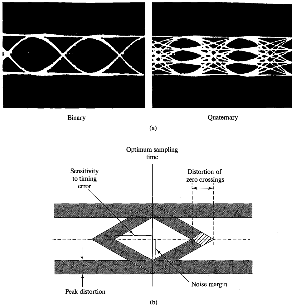
Figure 10.8 Eye patterns. (a) Examples of eye patterns for binary and quaternary PAM and (b) the effect of ISI on eye opening.
