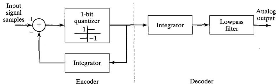
Figure 7.23 Delta modulation.
