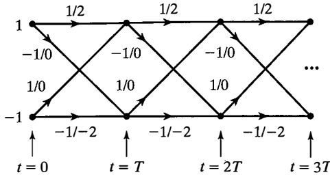
Figure 10.17 Trellis for duobinary partial response signals.
