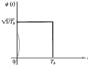
Figure 8.6 Unit energy basis function for binary PAM.
