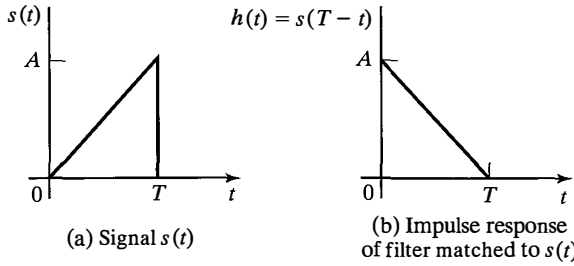
Figure 8.28 Signal s(t) and filter matched to s(t) .
