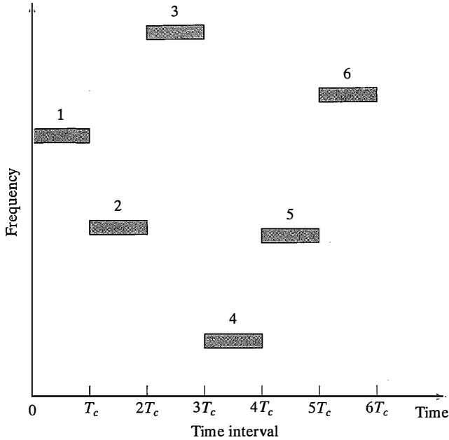
Figure 15.9 An example of an FH pattern.
