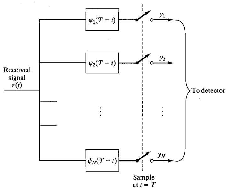
Figure 8.36 Matched-filter-type demodulator.
