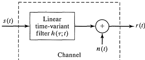
Figure 1.9 Linear time-variant filter channel with additive noise.
