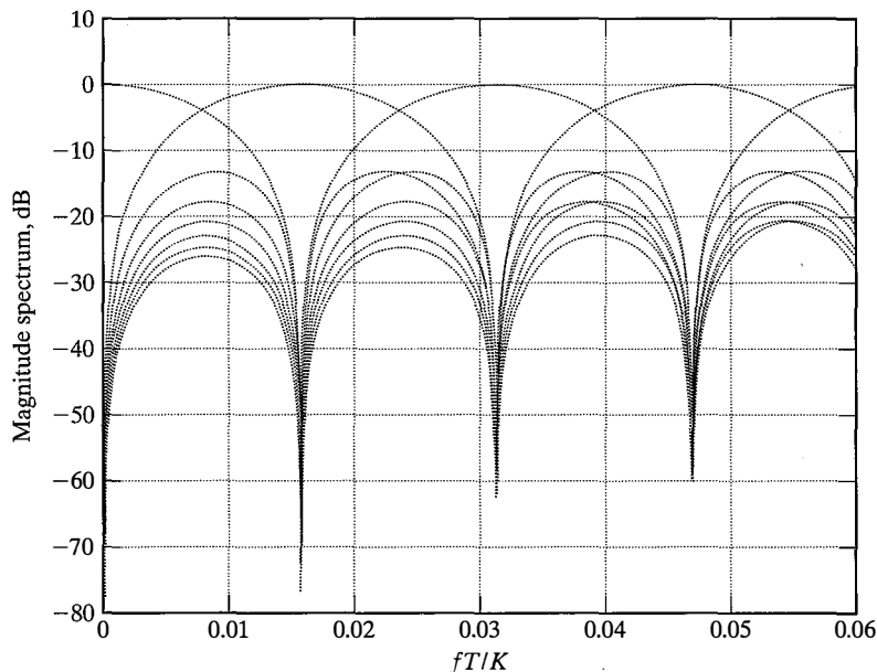
Figure 11.6 An example of the magnitude of the frequency response of adjacent subchannel filters in OFDM system for f \in (0, 0.06\frac{\lambda}{T}) and K = 64 . (From Cherubini et al. (2002) IEEE.)
