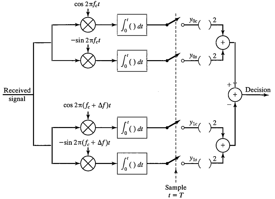
Figure 9.14 Demodulation and square-law detection of binary FSK signals.
