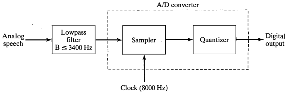
Figure 7.19 A general speech encoder.
