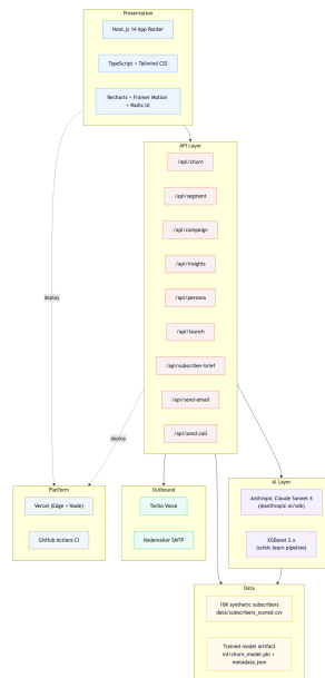
Figure 2. Layered technology stack. The Next.js presentation layer talks to a typed API layer that orchestrates the AI layer (Claude + XGBoost), the data layer (synthetic CSV + serialized model artifact), and outbound channels (Twilio, Nodemailer). The whole application deploys to Vercel from GitHub.
