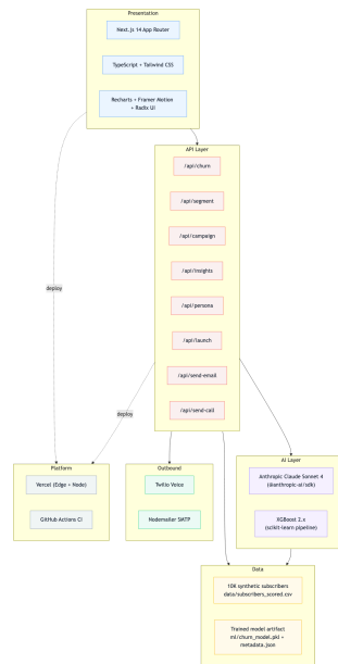
Figure 2. Layered technology stack. The Next.js presentation layer talks to a typed API layer that orchestrates the AI layer (Claude + XGBoost), the data layer (synthetic CSV + serialized model artifact), and outbound channels (Twilio, Nodemailer). The whole application deploys to Vercel from GitHub.
