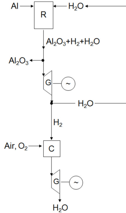
Figure 9: Simplified Overview of Metal-Water Propulsion System (R = metal-water reactor, G = steam generator, C = hydrogen combustion chamber) [8]
