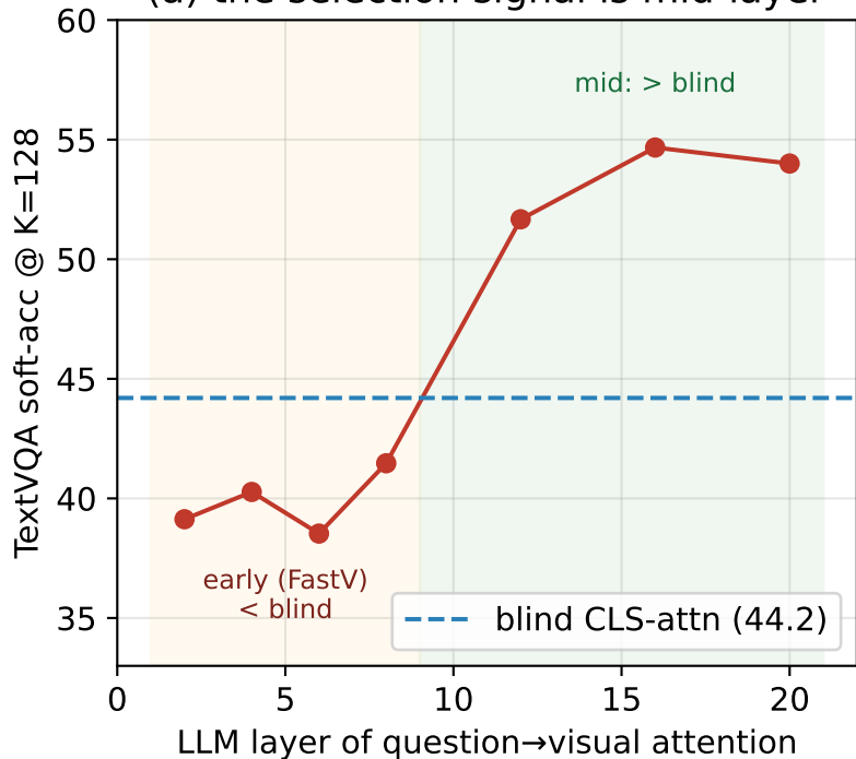
(a) the selection signal is mid-layer
