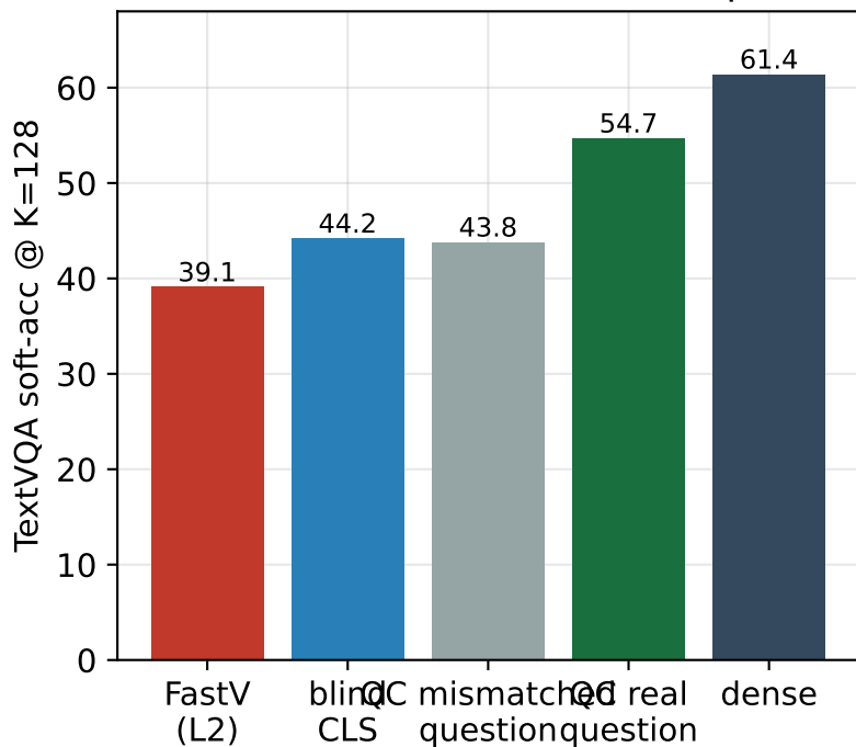
(b) the gain is question-conditioned (mismatched \approx blind; 104% from question)
