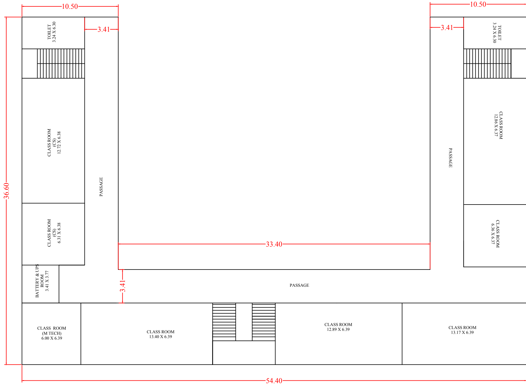
ACADEMIC BLOCK II (CS/IT BLOCK) SECOND FLOOR
