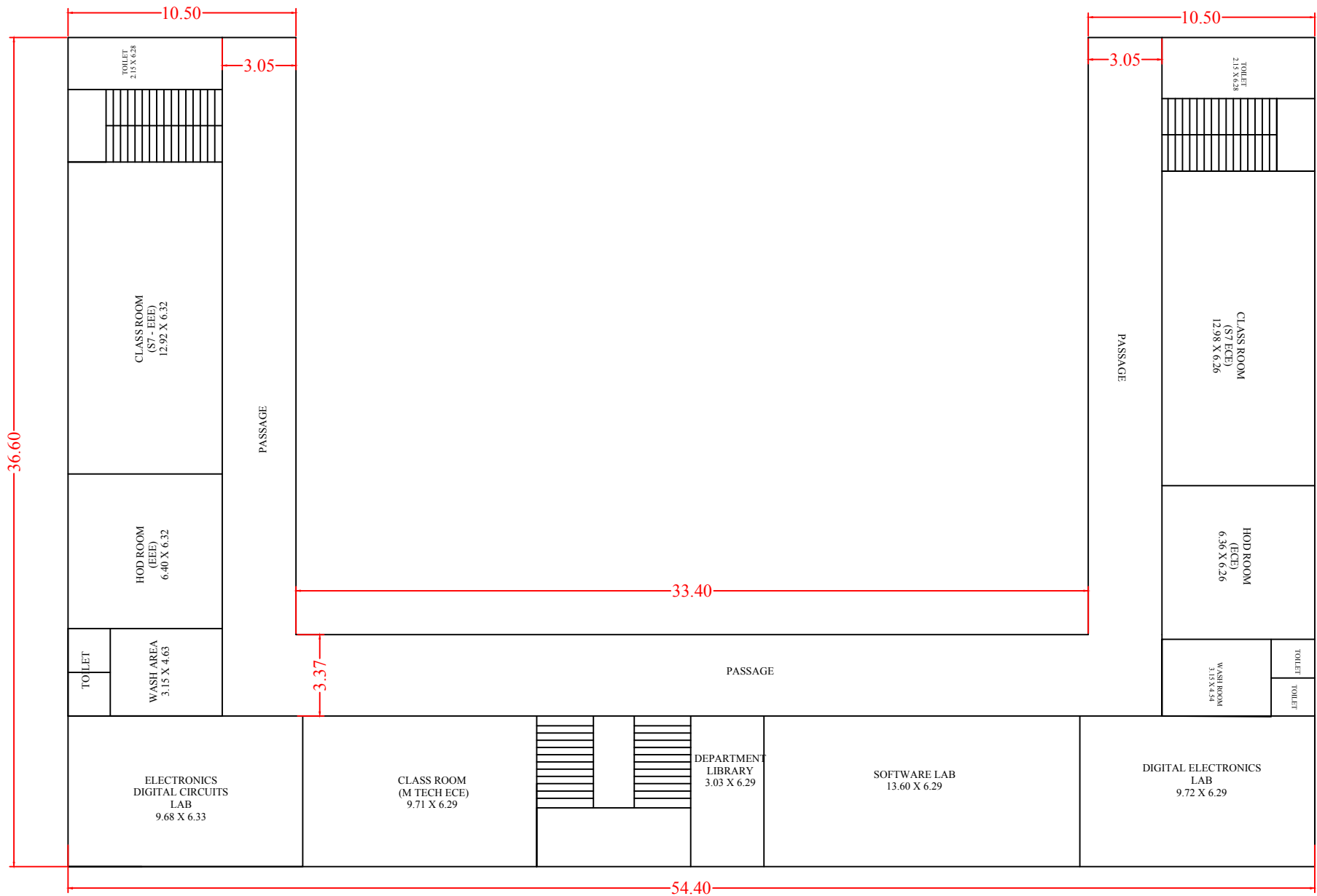
ACADEMIC BLOCK I (EEE/ECE BLOCK) FIRST FLOOR
