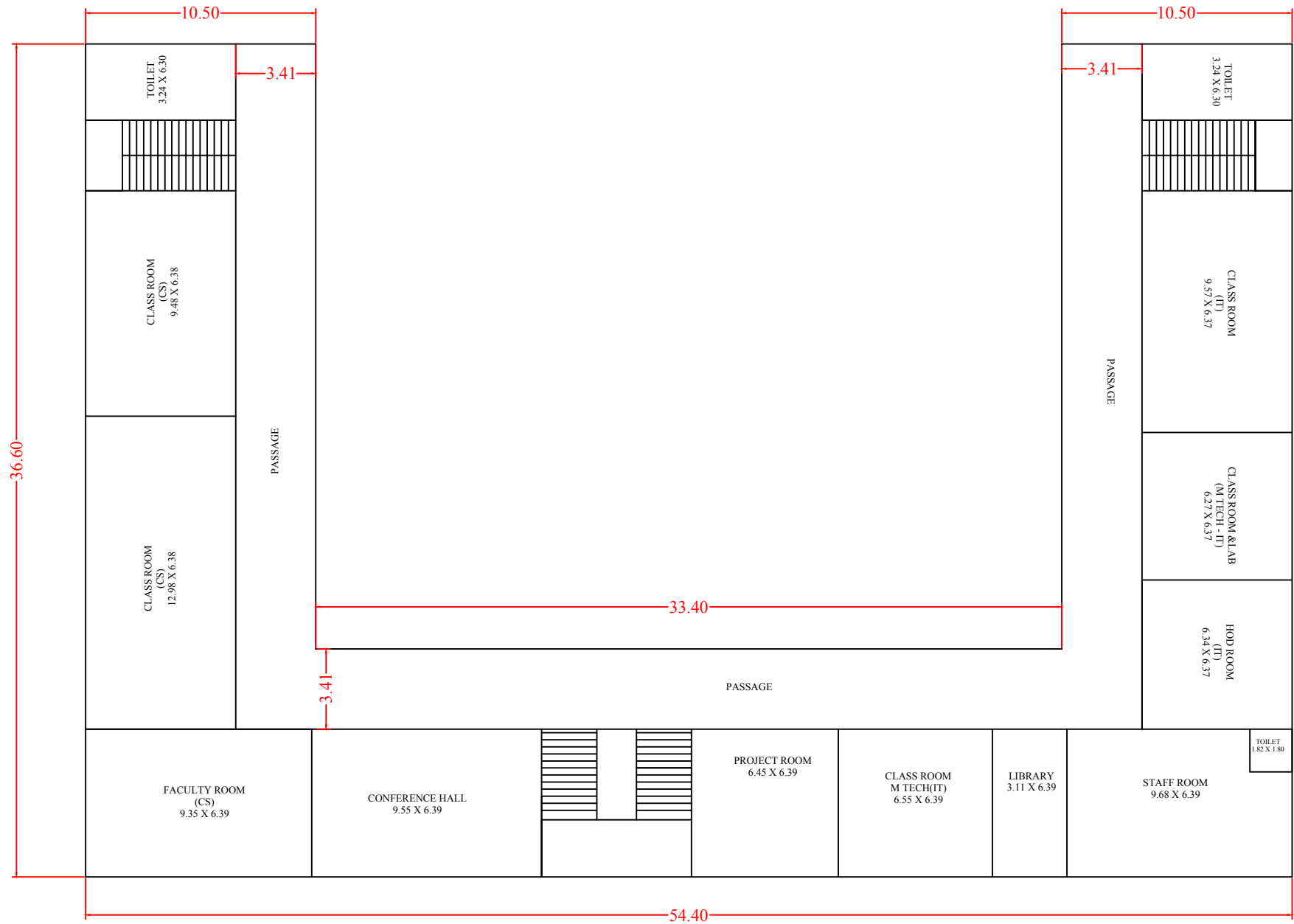
ACADEMIC BLOCK II (CS/IT BLOCK) FIRST FLOOR
