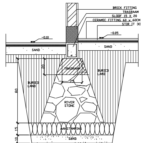
FOUNDATION DETAIL PIECES B SCALE 1:20
