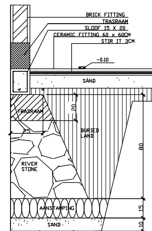
FOUNDATION DETAIL PIECES A SCALE 1:20
