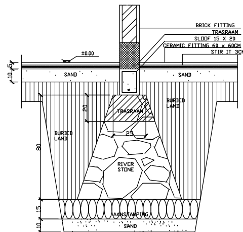
FOUNDATION DETAIL PIECES C SCALE 1:20
