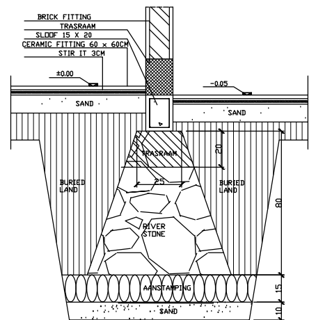
FOUNDATION DETAIL PIECES D SCALE 1:20
