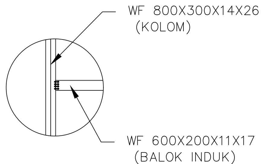
DETAIL IV
