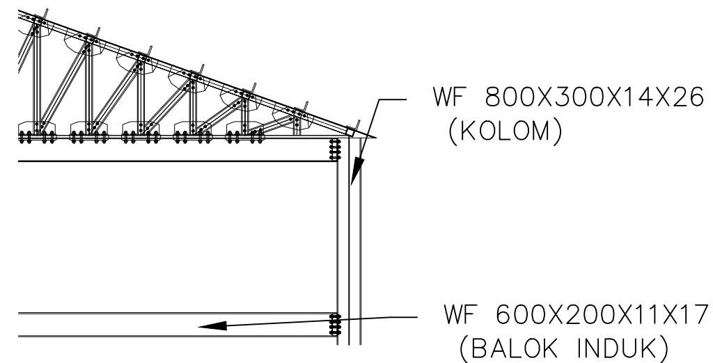
DETAIL II
