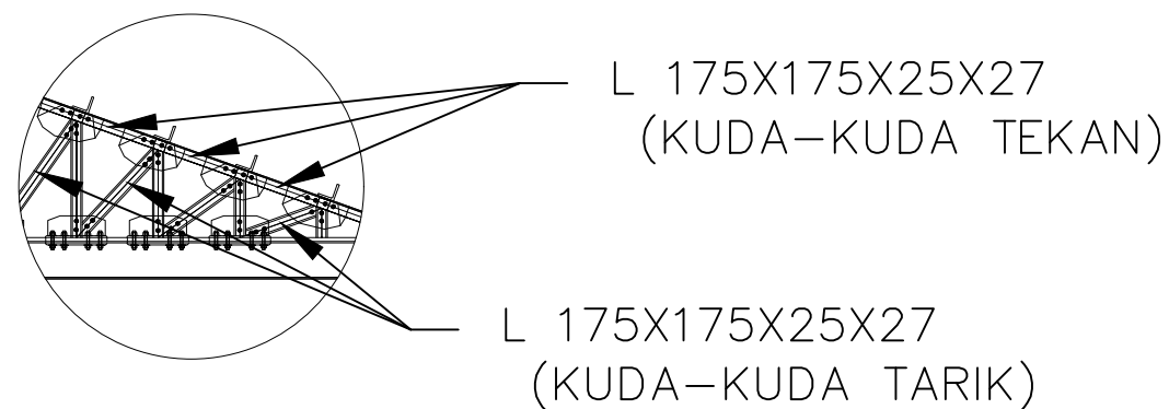
DETAIL I
