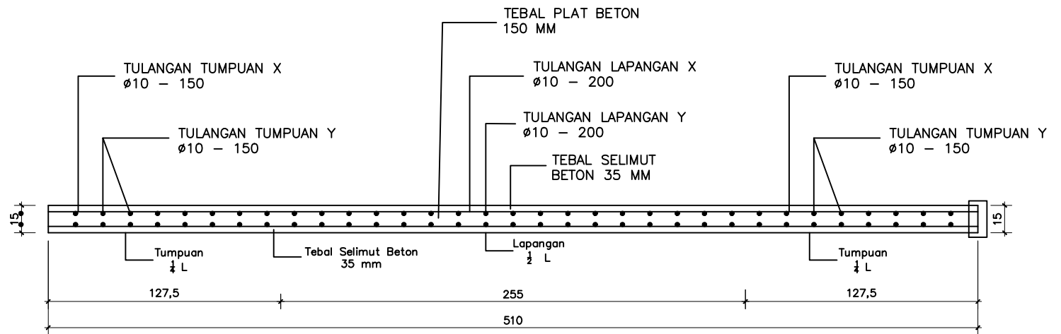
Potongan Floor Slab X LT 2-4 SKALA 1 : 100
