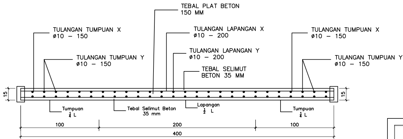
Potongan Floor Slab X LT 2-4 SKALA 1 : 100
