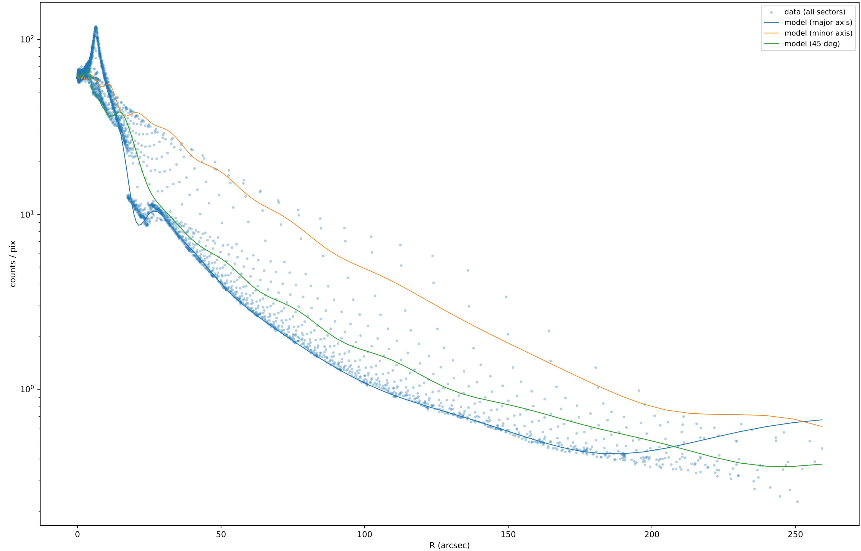
sombbrero_f200: radial profile data vs model (absdev=0.0379)
