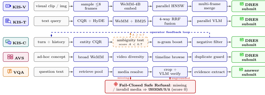
Fig. 2. Task-specific execution lanes for the 5 VBS modes. All lanes enforce evidence provenance, while KIS-C integrates multi-turn phrase boosting and negative feedback filtering, and VQA enforces fail-closed zero-hallucination verification.
