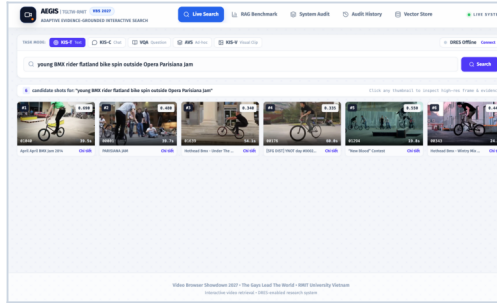
(a) KIS-T: Single-Turn Textual Retrieval (00000.mp4)
