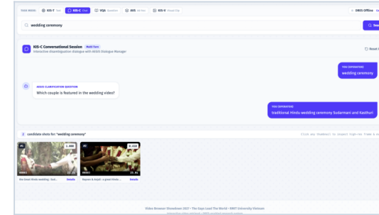
(b) KIS-C: Conversational Disambiguation (00003.mp4)
