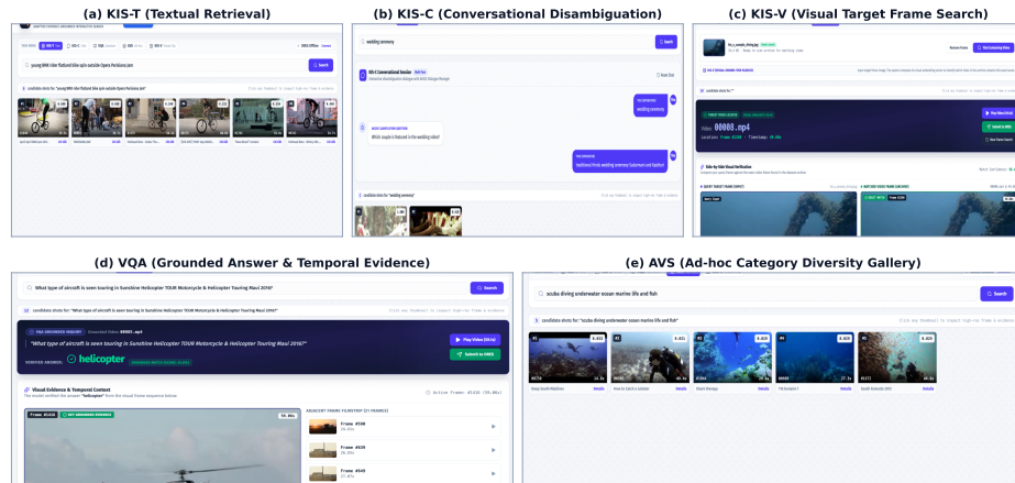
Fig. 3. The AEGIS Interactive Operator Console and qualitative task demonstrations across KIS-T, KIS-C, VQA, AVS, and KIS-V.
