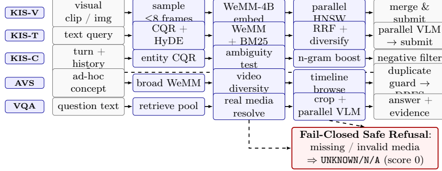
Fig. 2. Task-specific execution lanes for the 5 VBS modes. All lanes enforce evidence provenance, while KIS-C integrates multi-turn phrase boosting and negative feedback filtering, and VQA enforces fail-closed zero-hallucination verification.
