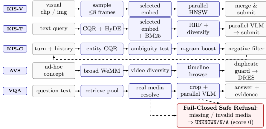
Fig. 2. Task-specific execution lanes for the 5 VBS modes. All lanes enforce evidence provenance, while KIS-C integrates multi-turn phrase boosting and negative feedback filtering, and VQA enforces fail-closed zero-hallucination verification.
