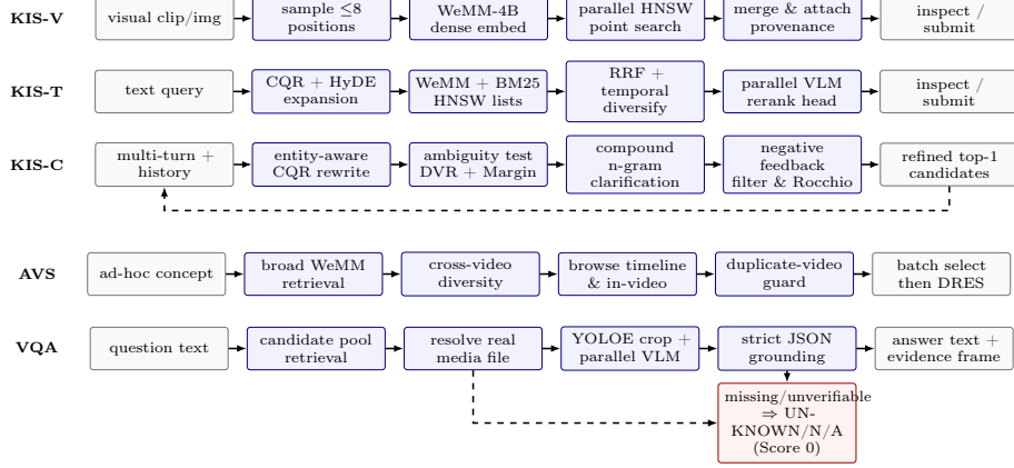
Fig. 2. Task-specific execution lanes for the 5 VBS modes. All lanes maintain strict evidence provenance, while KIS-C adds compound n -gram boosting and negative filtering, and VQA enforces fail-closed grounded execution.
