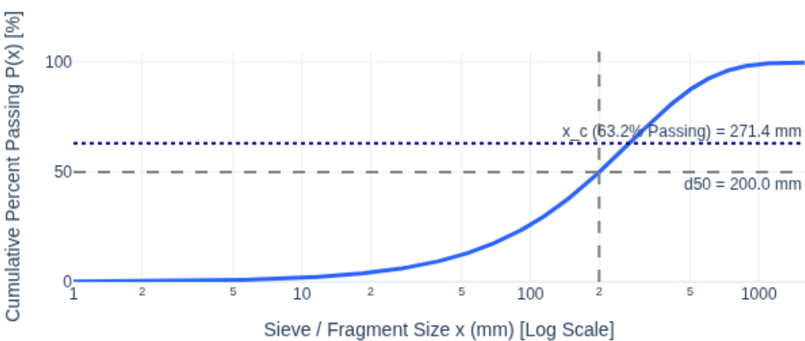
Kuz-Ram Fragmentation Curve (Percent Passing vs Size)
