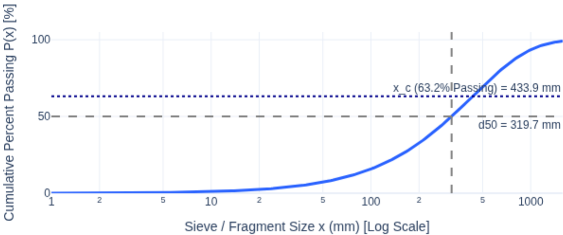
Kuz-Ram Fragmentation Curve (Percent Passing vs Size)
