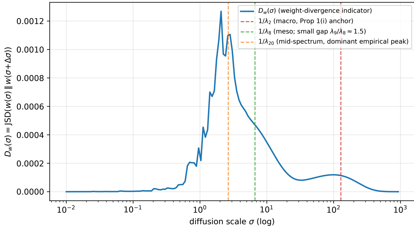
Empirical anchor for Proposition 1(i): HSBM r = 200 (seed 42), kNN-of-Poincaré-embedding Laplacian, focus = node 0
