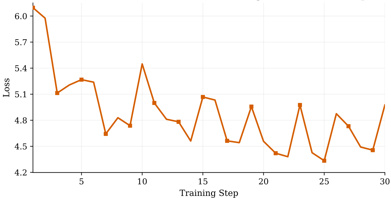
LLaMA-3.1-8B MemRift + LoRA Training Loss (First 30 Steps)
