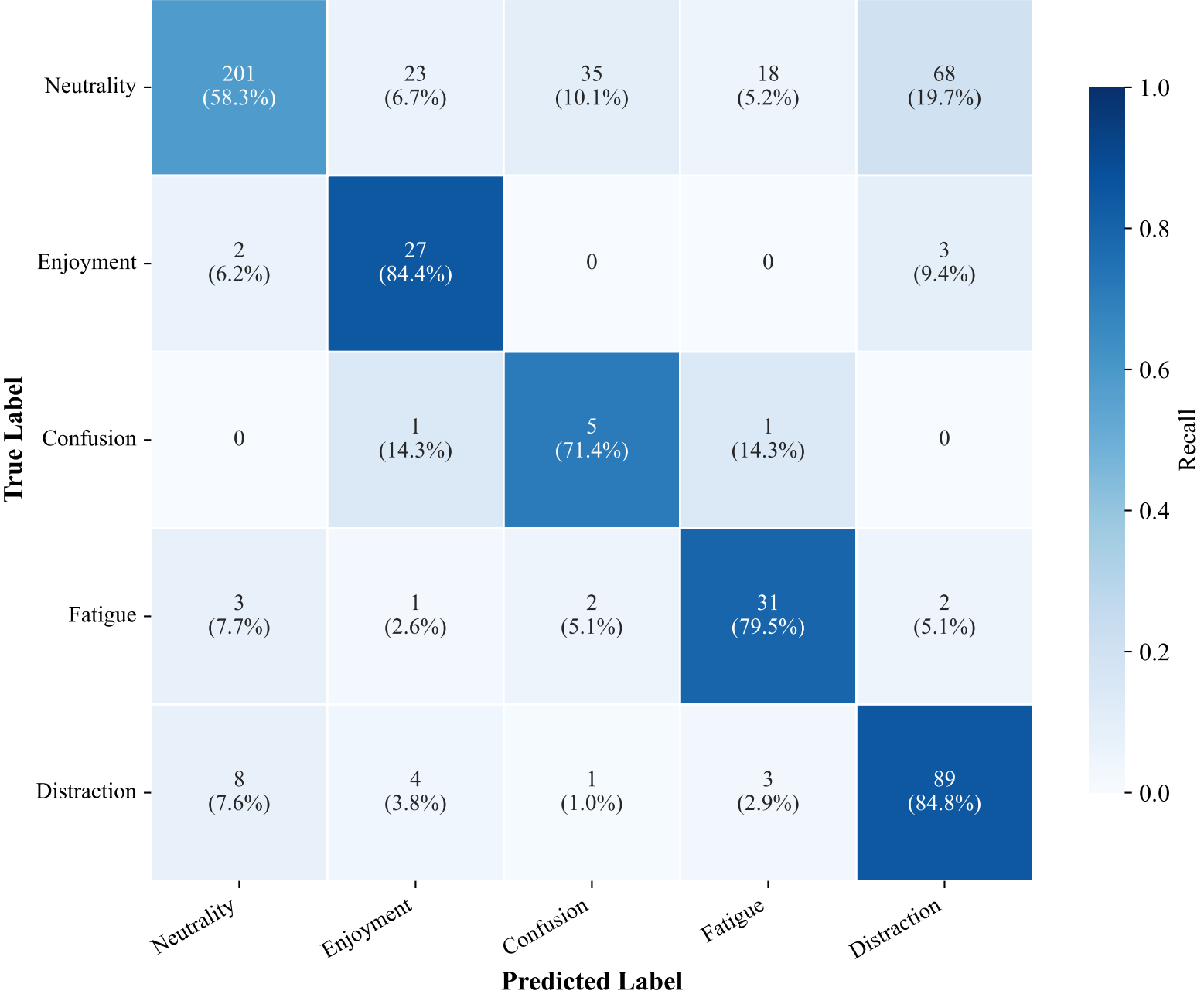
TTA + Bias Evaluation — Confusion Matrix WAR: 66.86% | UAR: 75.66%
